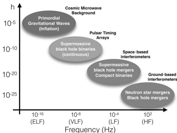
Рисунок 21.4 Schematic of astrophysical gravitational wave sources, as a function of wave frequency and wave strain.
