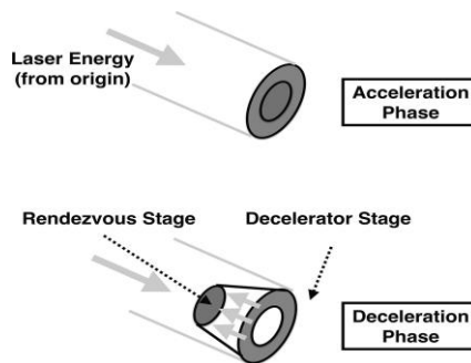
Рисунок 19.5 Schematic of Forward's (1984) two-sail concept for acceleration and deceleration phases. Laser light from the sail's origin (the Sun, thick arrows) impinges on both sails constructively during the acceleration phase, and destructively during deceleration, where the net momentum transfer on the rendezvous sail comes from photons deflected by the deceleration sail.
