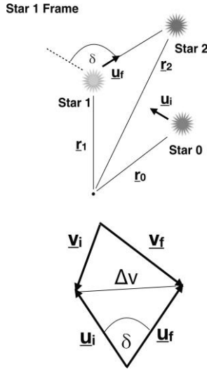
Рисунок 19.6 The slingshot manoeuvre, or gravitational assist. Top: The gravitational assist in the rest frame of star 1. Beginning from star 0, the probe achieves a velocity \mathbf{u}_i in star 1's rest frame, and leaves star 1 towards star 2 with velocity \mathbf{u}_f , with the same magnitude. Bottom: Comparing lab frame velocities ( \mathbf{v}_i, \mathbf{v}_f ) to the velocity in the frame of star 1.
