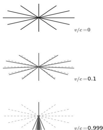
Рисунок 19.7 Illustrating relativistic aberration. Light is emitted by sources at rest along radial lines of sight towards our spacecraft at rest (top figure). Emitters from slightly behind these positions will still be visible from an observer travelling on the spacecraft at 0.1c (middle). At highly relativistic velocities, the observer's field of view becomes close to 360^\circ (bottom).
