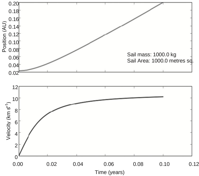
Рисунок 19.4 The position and velocity evolution of a 1 ton solar sail (area 1,000 \text{m}^2 ) as it accelerates away from the Sun, from an initial distance of 5 solar radii.
