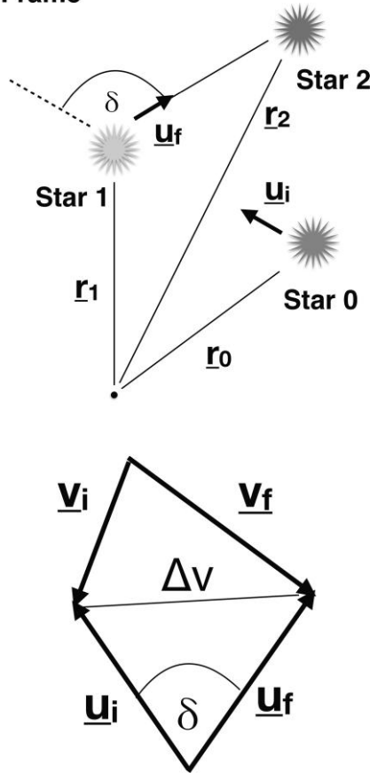
Рисунок 19.6 The slingshot manoeuvre, or gravitational assist. Top: The gravitational assist in the rest frame of star 1. Beginning from star 0, the probe achieves a velocity \mathbf{u}_i in star 1's rest frame, and leaves star 1 towards star 2 with velocity \mathbf{u}_f , with the same magnitude. Bottom: Comparing lab frame velocities (\mathbf{v}_i, \mathbf{v}_f) to the velocity in the frame of star 1.
