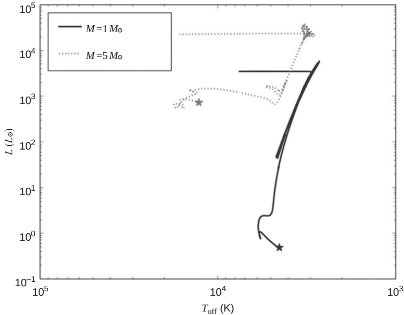
Рисунок 10.3 The evolution of a 1M star (solid line) and a 5M star (dotted line) on the HR diagram. We begin the tracks with both stars on the main sequence (through the subgiant branch to the red giant branch (RGB). Once the indicated by the star symbols). The 1M star evolves along and off the main star begins fusing helium in its core, it drops back down and joins the asymptotic giant branch (AGB), which closely tracks the RGB. After reaching the tip of the AGB (when helium burning in the core ceases), the star evolves towards the planetary nebula/white dwarf phase (not plotted). The 5M from the main sequence to the RGB (through the Hertzsprung Gap), and executes M star jumps rapidly across a ‘blue loop’ before joining the AGB, as it is able to begin helium fusion into carbon before it leaves the RGB. Data generated by the MESA Isochrones and Stellar Tracks project using the MESA stellar evolution code.
