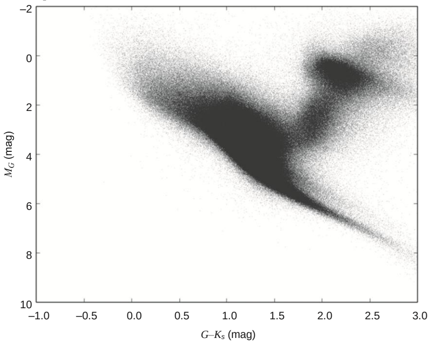
Рисунок 10.2 The Hertzsprung Russell Diagram, generated from the Gaia Data Release 1. Note that effective temperature ( x -axis, where spectral colour is used as a proxy) increases from right to left. Most stars are located along the main
