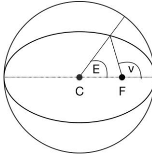
Рисунок 4.2 Эксцентриситет и истинная аномалия кеплеровской орбиты. Bodies orbit in ellipses around the focus (F). The eccentric anomaly describes the angle that the orbiting body would make with the centre of the ellipse (C) if the body executed a circular orbit. Hence, the eccentric and true anomaly are equivalent when the orbit is circular.
