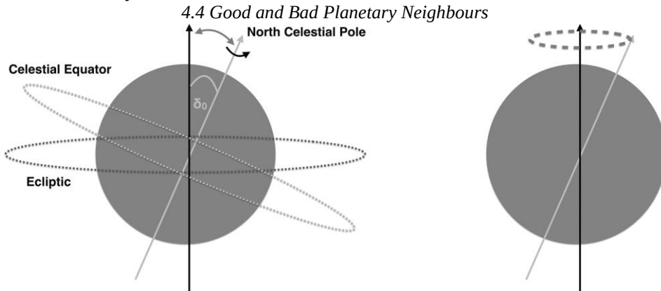
Рисунок 4.11 The obliquity \delta_0 of the Earth. There are two Milankovitch cycles associated with the obliquity. In the first, the magnitude of the obliquity can change (left). In the second, the obliquity precesses (right).
