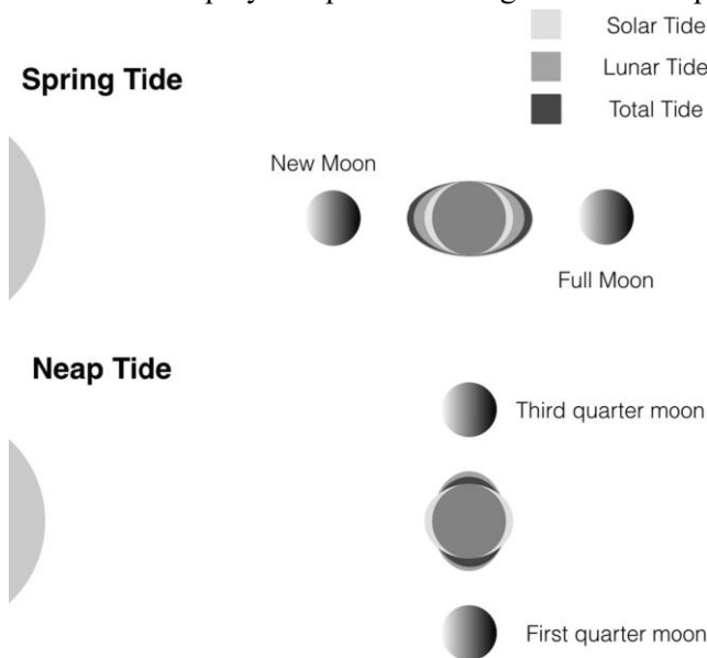
Рисунок 4.14 The spring and neap tides. Depending on the relative orientation of the Sun and Moon, the lunar and solar tides can co-add to produce the spring tide, or add orthogonally to produce the neap tide.
