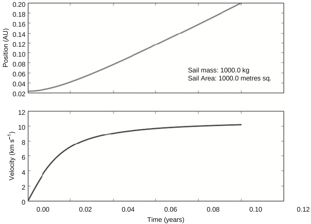
Рисунок 19.4 The position and velocity evolution of a 1 ton solar sail (area 1,000 \text{ m}^2 ) as it accelerates away from the Sun, from an initial distance of 5 solar radii.
