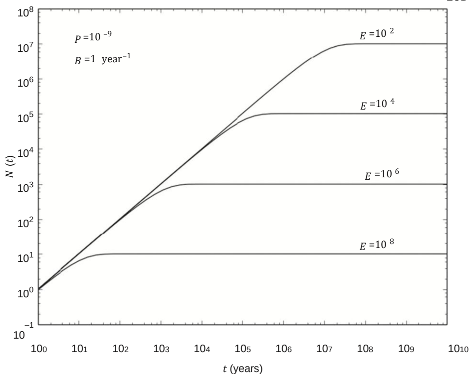
Рисунок 14.1 The number of communicating civilisations as a function of time, given E individuals causing self-destruction with a probability of P per individual per year. The civilisation birth rate B is fixed at one per year.
