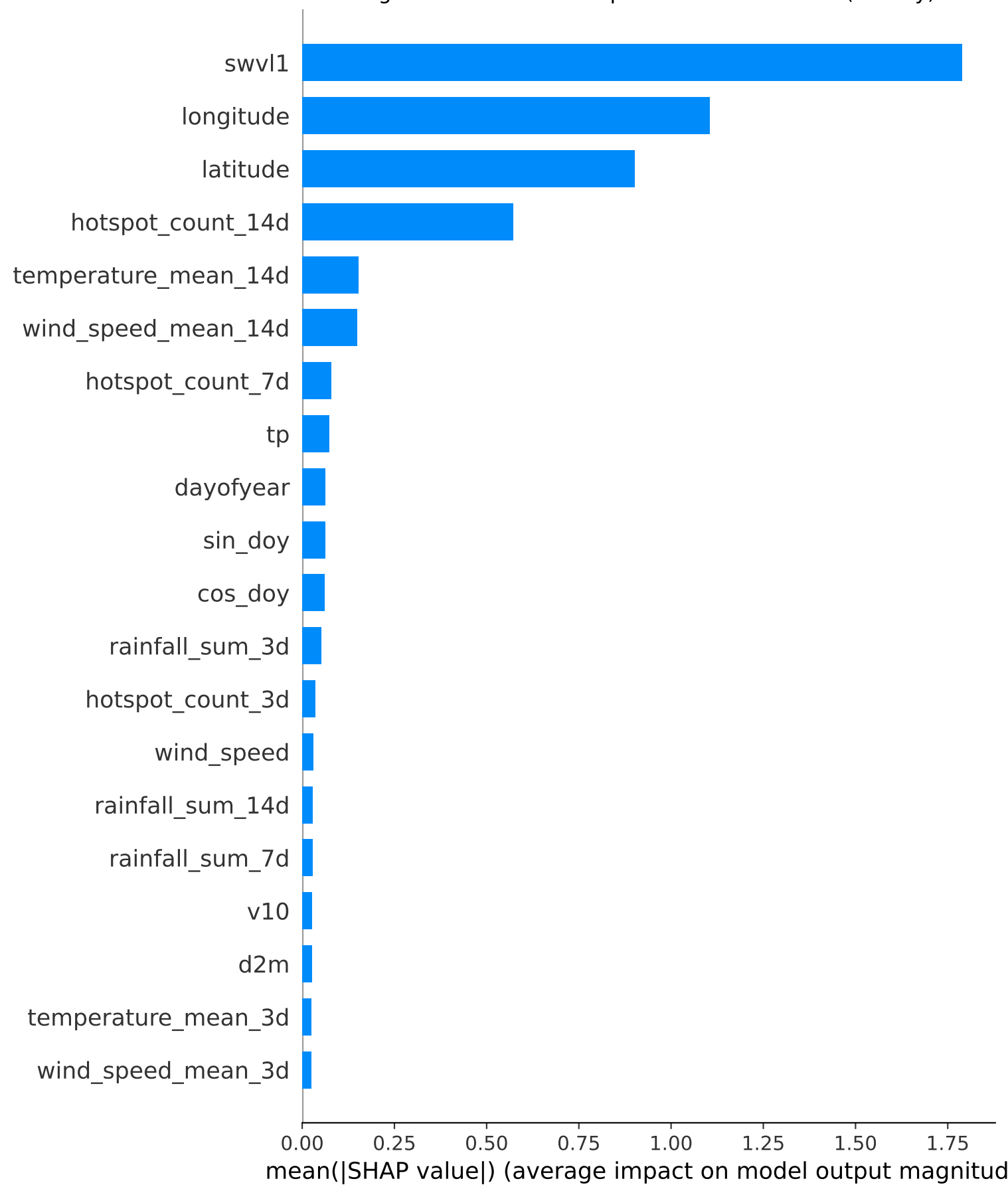
Fig. 6. SHAP Feature Importance for XGBoost (14-day)
