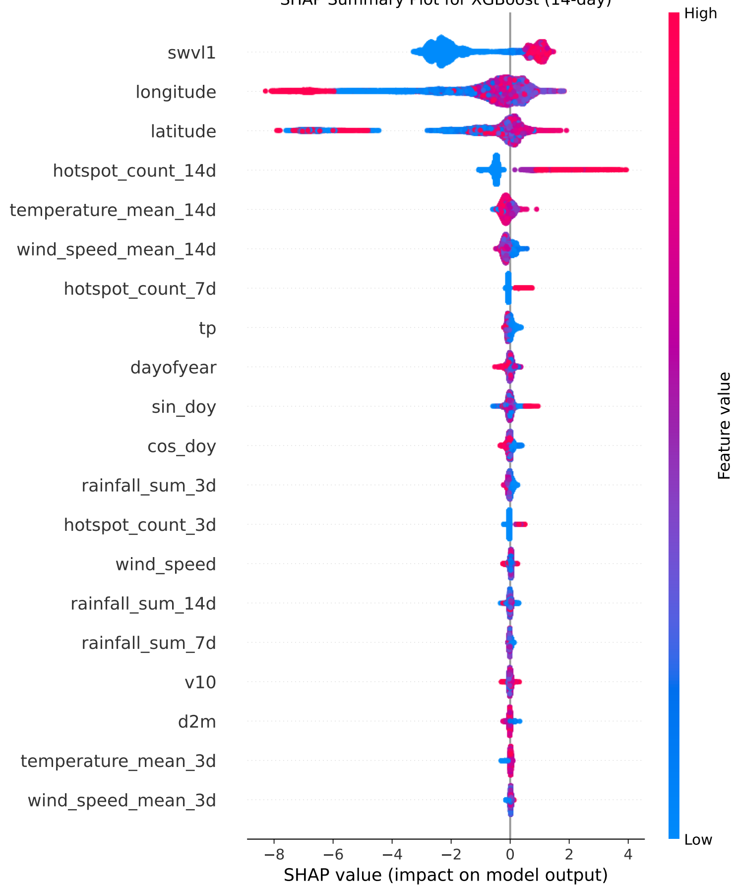
SHAP Summary Plot for XGBoost (14-day)
