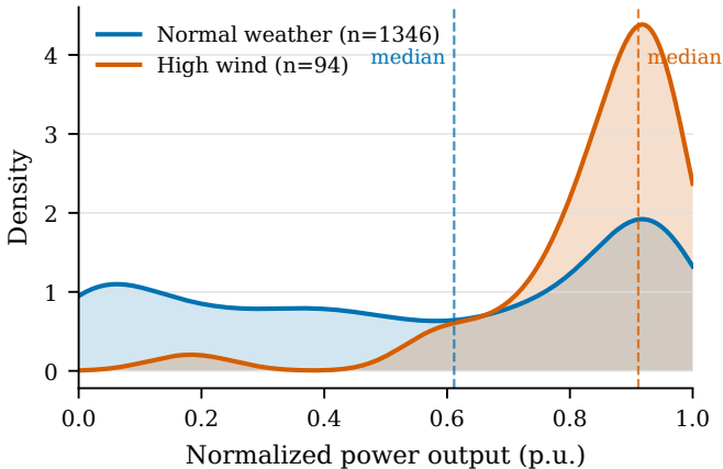
Power distribution in high-wind and normal weather
