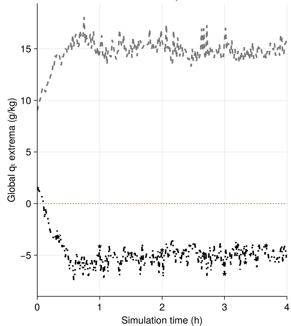
Fine: \Delta x = 10 m, \Delta z = 5 m
