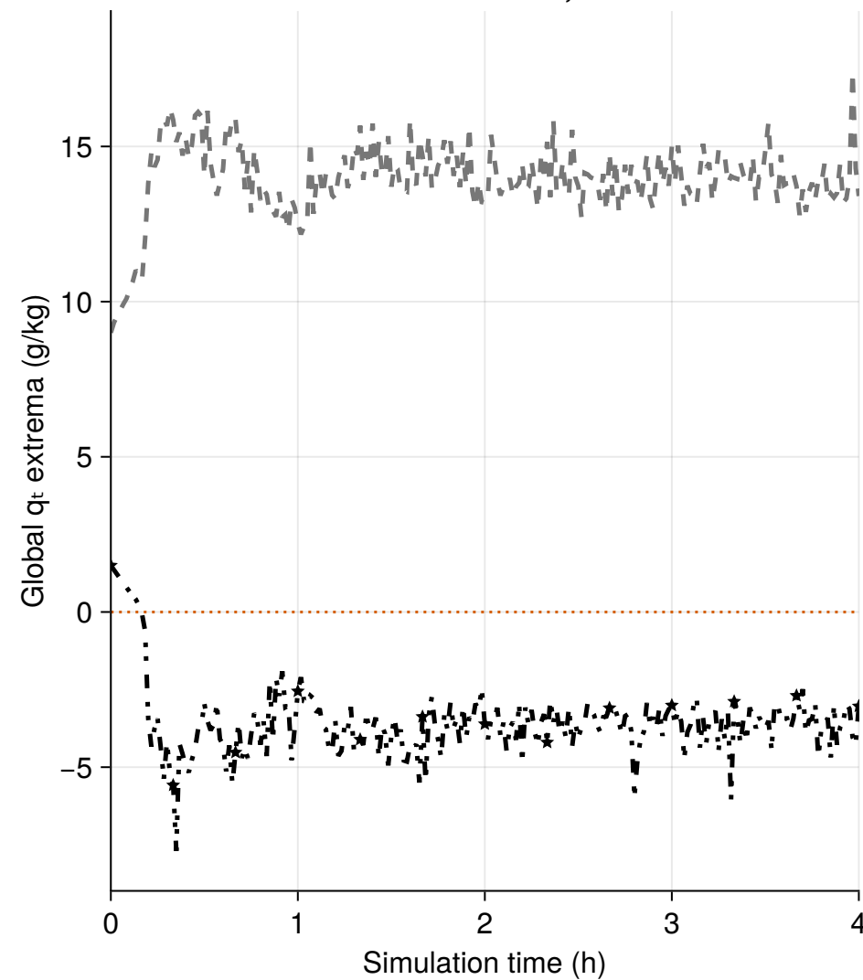
Canonical: \Delta x = 35 m, \Delta z = 5 m
