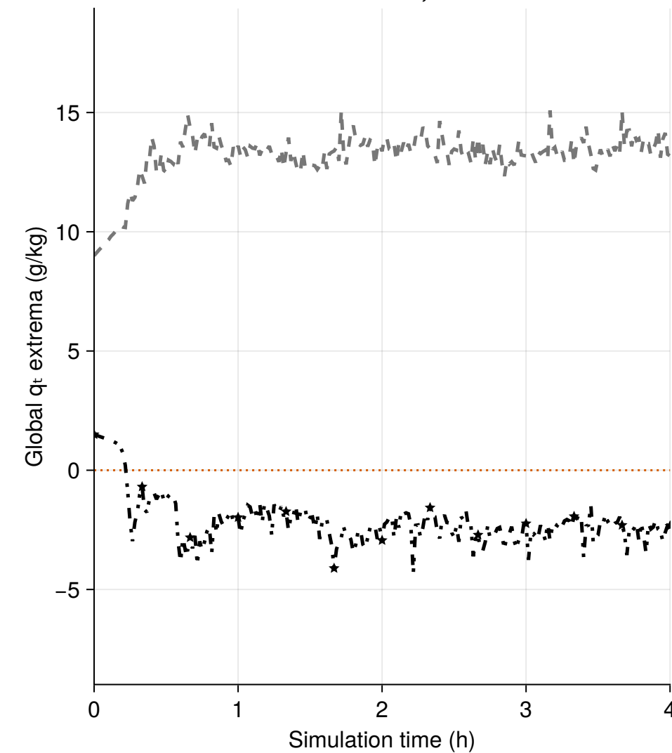
Coarse: \Delta x = 80 m, \Delta z = 20 m
