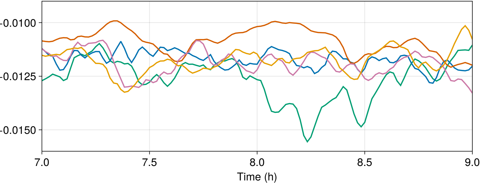
Surface heat flux
