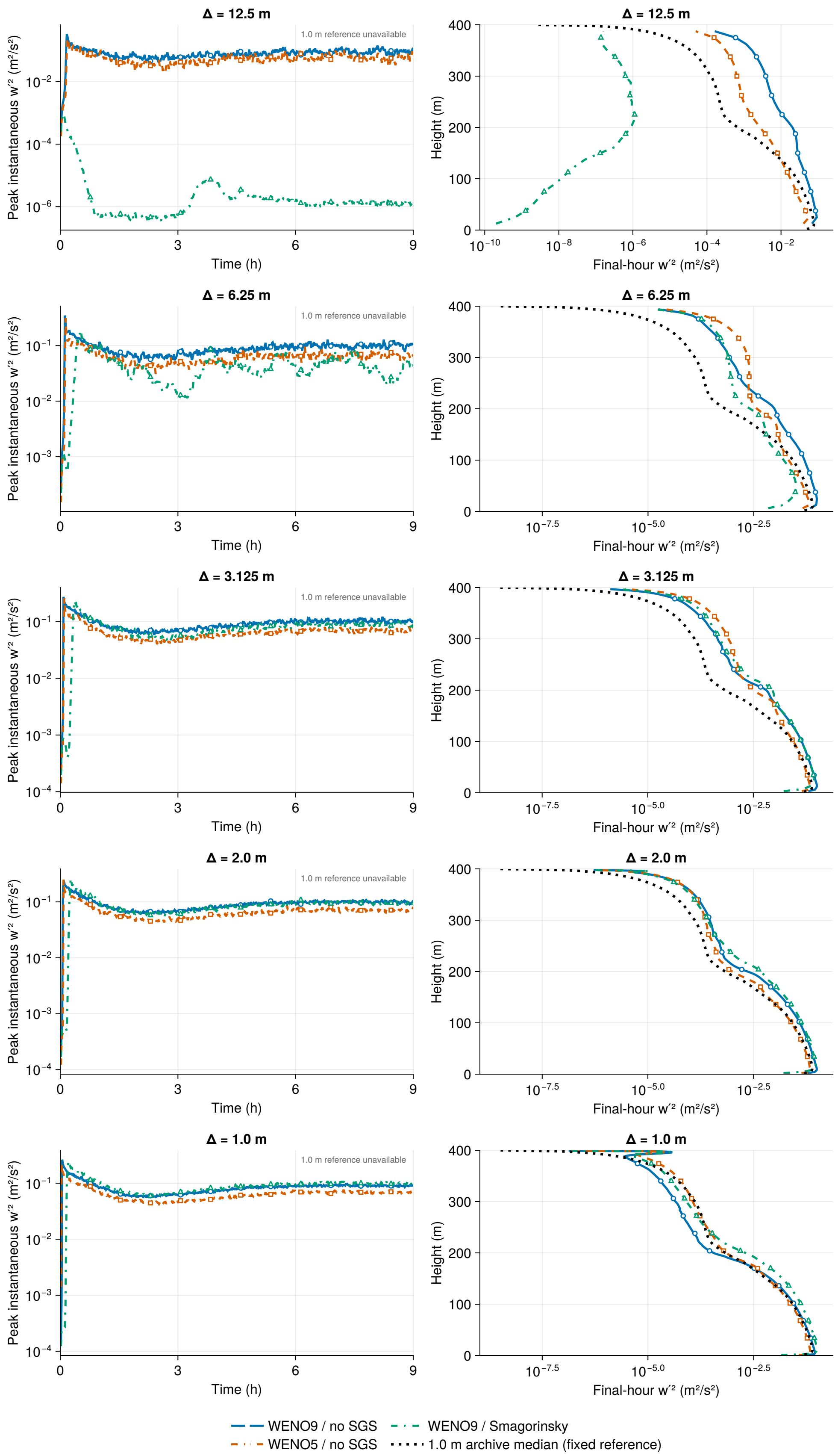
Logarithmic variance axes distinguish weak resolved motions from sustained turbulence. Left: instantaneous profile maxima; right: 8–9 h means. Black dots: fixed 1.0 m median (right only). No archived peak-variance time series. Nonpositive values omitted without a substituted floor.
