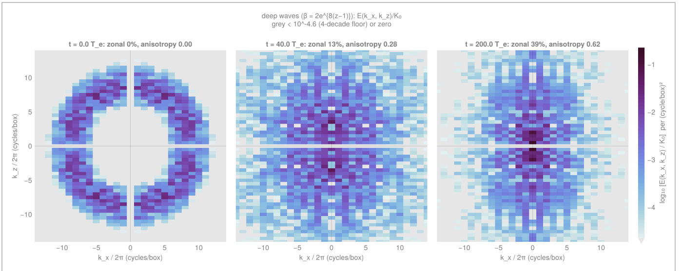
Deep waves, same diagnostic. E(k_x, k_z)/K_0 for the deep-wave member (same ring initial condition, seed 1, 256 2 ) at 0, 40 and 200 T e , on the same colour scale as the shallow-wave figure above: log 10 limits -4.65 to -0.65 , shared by the shallow, deep and wave-free spectra, grey below the four-decade floor or exactly zero, so the two figures compare cell by cell. The spectrum is a Fourier ( x ) \times sine ( z ) decomposition of the streamfunction over the whole column between the walls: k_z/2\pi = n/2 counts vertical half-wavelengths across the domain, the k_z = 0 row is empty because the sine basis has no n = 0 mode, and a given ( k_x, k_z ) cell mixes contributions from every depth rather than describing waves at one level. No dumbbell is drawn: \beta_{\text{eff}}(z) = \partial z u^* = 2e^{\{8(z-1)\}} varies by a factor of about 3000 over the depth, so a constant- \beta Rhines estimate has no single value here. Energy leaves the ring and concentrates in and next to the exact-zonal k_x = 0 column at low |k_z| (about 0.5–2 cycles per box): exact-zonal fraction 0 \rightarrow 13% \rightarrow 39% and anisotropy 0.00 \rightarrow 0.28 \rightarrow 0.62, whereas with shallow waves the energy collects at the dumbbell poles off the k_x = 0 axis (exact-zonal 5%, anisotropy 0.70 at 200 T e ). Single realization at one grid; the deep-wave jet statistics are seed-sensitive and change by roughly 10–20% across the higher-resolution comparisons (exact-zonal fraction 0.38 at 512 2 and 0.45 at 1024 2 at 200 T e ; see REPORT_resolution.md ). Figure final_spectra_deep_heatmap.png ( analysis/wc25_vallis2d/figures.jl , spectra_only=true , the same render as the shallow figure).
