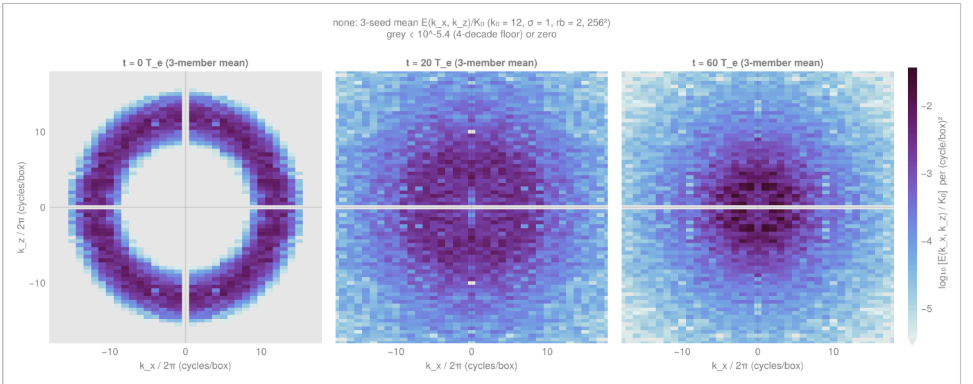
Wave-free ensemble mean (three seeds, same ring): isotropic collapse toward small K with no preferred direction; exact-zonal fraction 0.06 \pm 0.03 from the condensate's random projection onto the x-mean. Figure final_ensemble_spectra_none_heatmap.png . Heatmap: spectral density per (\text{cycle/box})^2 , normalized by the initial energy K_0 , one cell per lattice mode ( k_x/2\pi integer, k_z/2\pi = n/2 for the wall sine basis), \log_{10} colour on a perceptually uniform sequential map with limits shared across the panels and families being compared; cells more than four decades below the shared maximum, or exactly zero, are grey. No interpolation. The earlier filled-contour version is kept as final_ensemble_spectra_none.png .
