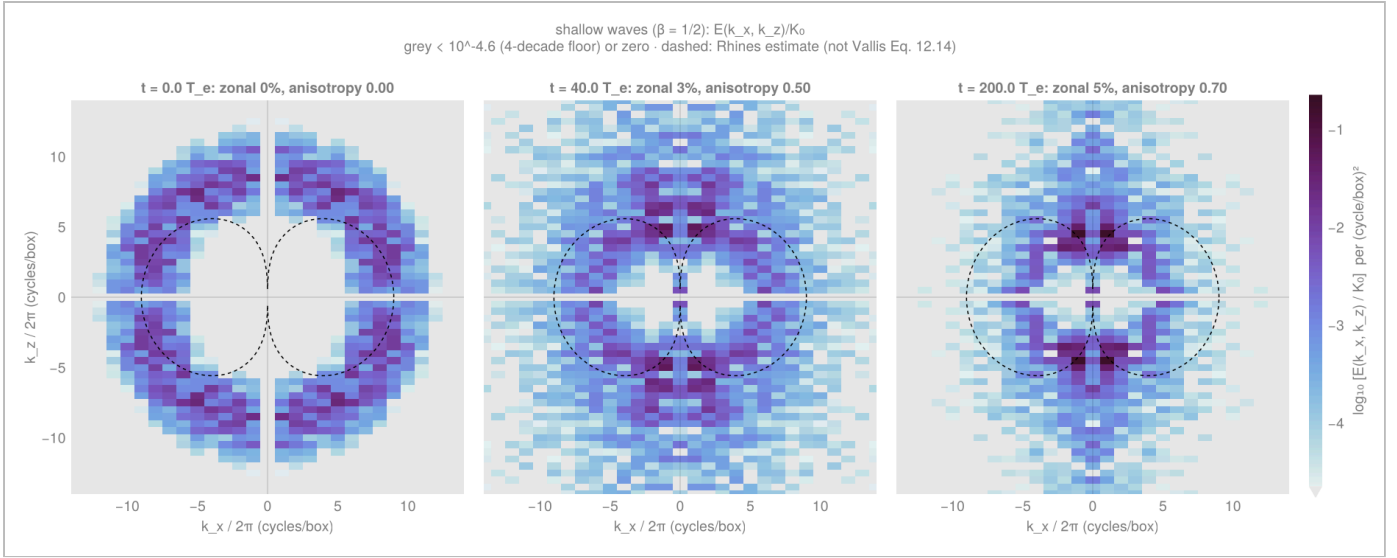
Shallow waves, the Fig. 12.3 analogue. E(k_x, k_z)/K_0 at 0, 40 and 200 T e with a Rhines-scale estimate K^2 = \beta |\cos \theta| / u'_{\text{rms}}(t) dashed (a velocity-based estimate using the instantaneous rms speed, not the textbook \varepsilon -based boundary of Vallis Eq. 12.14, whose shape differs). The energy leaves the ring and becomes concentrated near the k_z axis; the dashed curve is too large to trace the observed depleted region. It remains near a maximum radius of 9 cycles/box as total rms speed changes little. The spectral concentrations lie ( |k_x| \approx 3 , k_z \approx 4-8 cycles at 40 T e ; |k_x| \leq 2 , k_z \approx \pm 4-5 at 200 T e ). Anisotropy index 0.00 \rightarrow 0.50 \rightarrow 0.70; exact-zonal fraction 0 \rightarrow 3% \rightarrow 5%. Figure final_spectra_shallow_heatmap.png . Heatmap: spectral density per (cycle/box) 2 , normalized by the initial energy K_0 , one cell per lattice mode ( k_x/2\pi integer, k_z/2\pi = n/2 for the wall sine basis), log 10 colour on a perceptually uniform sequential map with limits shared across the panels and families being compared; cells more than four decades below the shared maximum, or exactly zero, are grey. No interpolation. The earlier filled-contour version is kept as final_spectra_shallow.png .
