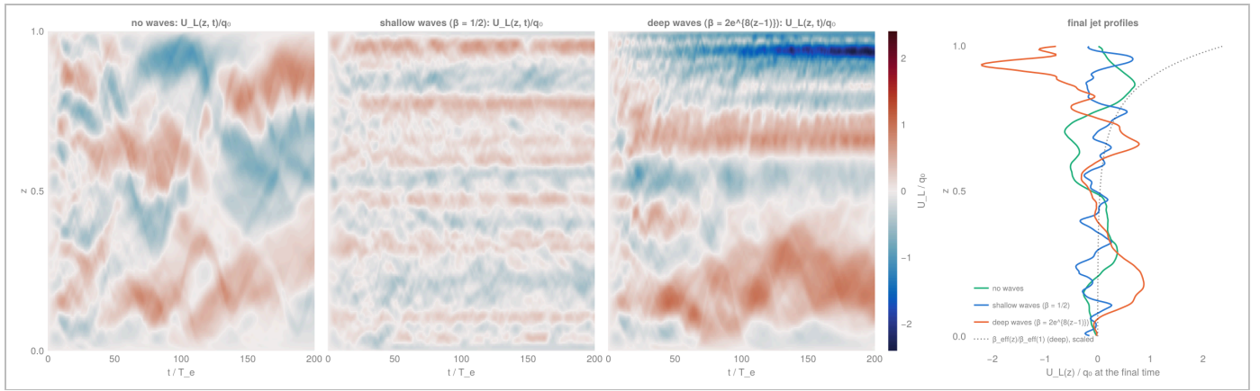
x-mean jets. U_L(z, t)/q_0 for no waves (left), shallow waves (middle) and deep waves (third), with final profiles at right. Shallow: many fine, weak bands (max 0.67 q_0 , wavelength \approx 0.09 ). Deep: a surface jet toward -x at z \approx 0.9 reaching -2.2 q_0 and interior jets toward +x near z \approx 0.65 and 0.2 (4 sign reversals, wavelength \approx 0.2 ), growing almost linearly in K_{\text{jet}}/K to 0.39 . Figure final_jets.png.
