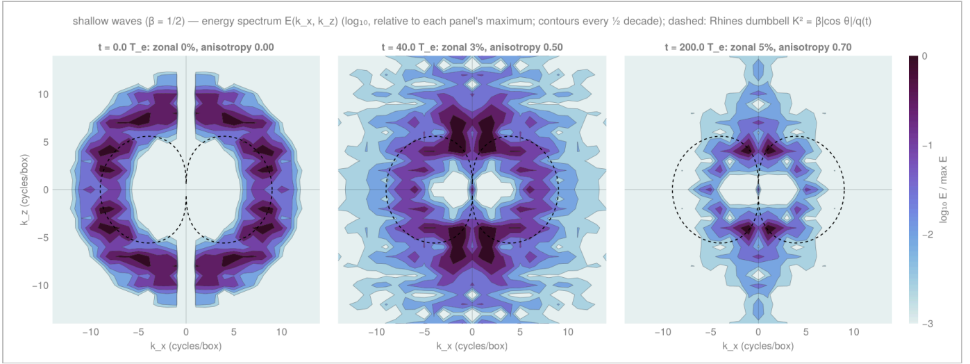
Shallow waves, the Fig. 12.3 analogue. E(k_x, k_z) ( \log_{10} , half-decade contours) at 0, 40 and 200 T e with a Rhines-scale estimate K^2 = \beta |\cos \theta| / q(t) dashed (a velocity-based estimate using the instantaneous rms speed, not the textbook \varepsilon -based boundary of Vallis Eq. 12.14, whose shape differs). The energy leaves the ring, avoids the dumbbell interior and collects at its poles ( |k_x| \lesssim 3 , k_z \approx 4-8 cycles at 40 T e ; |k_x| \lesssim 2 , k_z \approx \pm 4-5 at 200 T e ). Anisotropy index 0.00 \rightarrow 0.50 \rightarrow 0.70; exact-zonal fraction 0 \rightarrow 3% \rightarrow 5%. Figure final_spectra_shallow.png.
