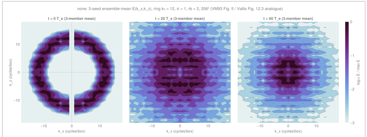
Wave-free ensemble mean (three seeds, same ring): isotropic collapse toward small K with no preferred direction; exact-zonal fraction 0.06 \pm 0.03 from the condensate's random projection onto the x -mean. Figure final_ensemble_spectra_none.png .
