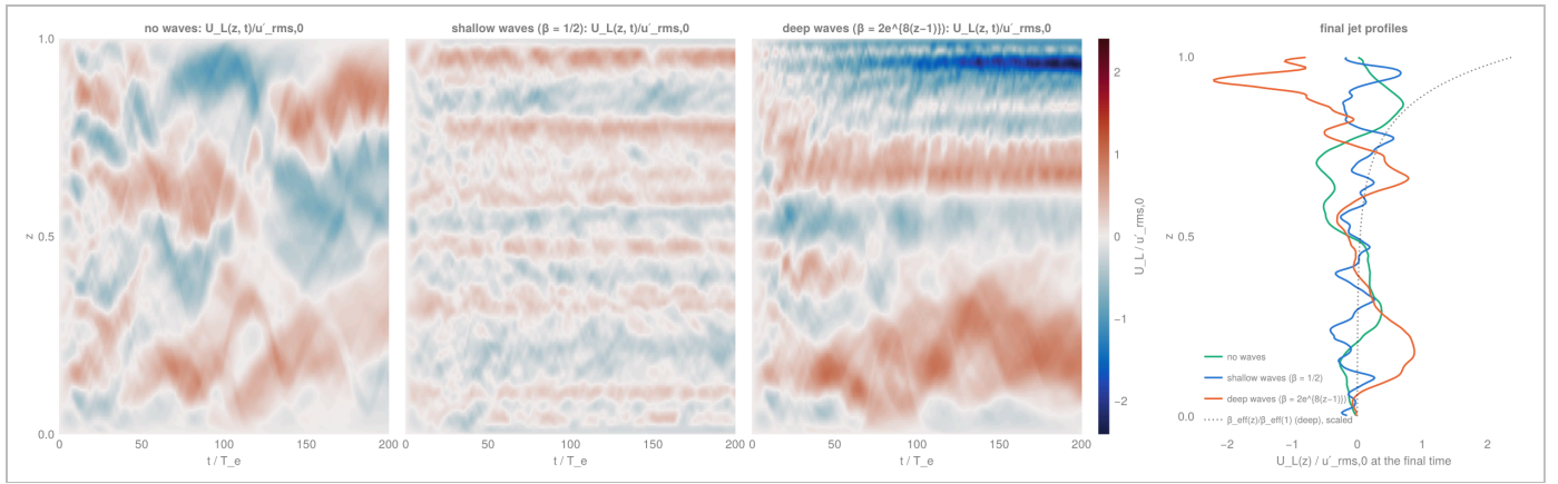
PROVISIONAL — VERY LOW RESOLUTION (256 2 / 256 3 and coarser). x-mean jets. U_L(z, t)/u'_{rms,0} for no waves (left), shallow waves (middle) and deep waves (third), with final profiles at right. Shallow: many fine, weak bands (max 0.67 u'_{rms,0} , wavelength \approx 0.09 ). Deep: a surface jet toward -x at z \approx 0.9 reaching -2.2 u'_{rms,0} and interior jets toward +x near z \approx 0.65 and 0.2 (4 sign reversals, wavelength \approx 0.2 ), growing almost linearly in K_{jet}/K to 0.39. Figure final_jets.png.
