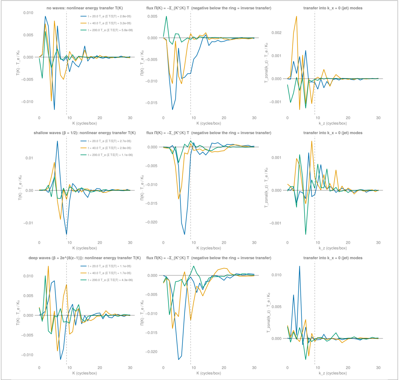
PROVISIONAL — VERY LOW RESOLUTION ( 256^2 / 256^3 and coarser). Spectral transfer. T(K) is negative at the ring ( K \approx 7-9 ) and positive at K \approx 4-6 , so the flux \Pi(K) = -\sum_{K' \leq K} T is negative below the ring: an inverse energy transfer, strongest at 20 T_e and weakening by 200 T_e ( \sum T/\sum |T| \approx 1e-5 , so the diagnostic is conservative). The transfer into k_x = 0 modes is 10\times larger with deep waves than with shallow waves and concentrated at k_z \approx 2-4 cycles. Figure final_transfer.png.
