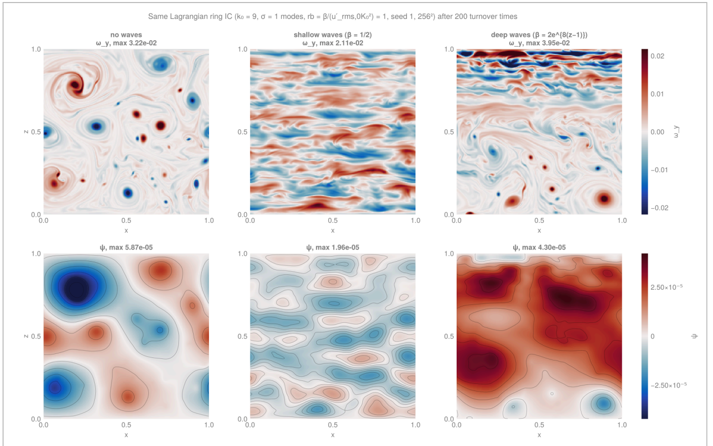
PROVISIONAL — VERY LOW RESOLUTION ( 256^2 / 256^3 and coarser). Three families at 200 T_e ( \omega_y top, \psi bottom, shared limits). No waves: Vallis Fig. 11.8 decay — coherent vortices, merger, a flat enstrophy landscape, energy centroid 2.6 cycles, enstrophy 14%. Shallow: x-elongated bands, centroid 5.1 cycles, enstrophy 39%. Deep: \beta dynamics in the upper third (where local \beta/(u'_{rms,0}K_0^2) exceeds \approx 0.1 ), 2-D vortices below z \approx 0.6 , and a mean streamfunction of one sign carrying the x-mean jet. Figure final_comparison_t200.png.
