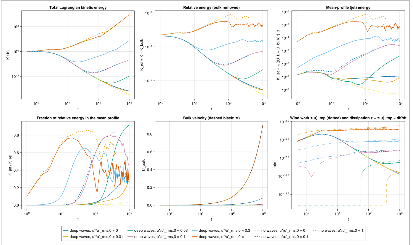
PROVISIONAL – VERY LOW RESOLUTION ( 256^2 / 256^3 and coarser). Energy budget. Total Lagrangian kinetic energy K/K_0 decays to 1.3e-3 at t = 400 with waves against 0.9e-3 without (top left); mean-profile energy K_{jet} (top right) grows at zero stress from t \approx 100 while the control's falls, and the fraction K_{jet}/K_{rel} (bottom left) reaches 0.40 at t = 1000 (control \leq 0.02 ). The bulk velocity follows \tau t exactly (bottom middle, momentum check), and the budget residual \epsilon = \tau(u)_{top} - dK/dt is positive at all times (implicit dissipation only removes energy). Figure final_energy.png.
