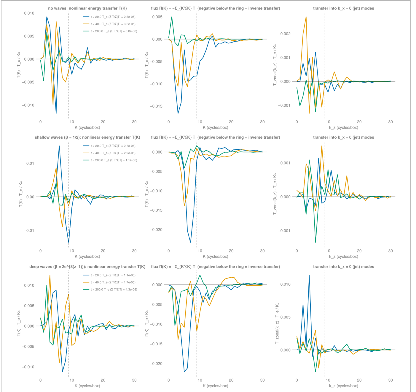
Spectral transfer. T(K) is negative at the ring ( K \approx 7-9 ) and positive at K \approx 4-6 , so the flux \Pi(K) = -\sum_{K' \leq K} T is negative below the ring: an inverse energy transfer, strongest at 20 T_e and weakening by 200 T_e ( \sum T/\sum |T| \approx 1e-5 , so the diagnostic is conservative). The transfer into k_x = 0 modes is 10x larger with deep waves than with shallow waves and concentrated at k_z \approx 2-4 cycles. Figure final_transfer.png .
