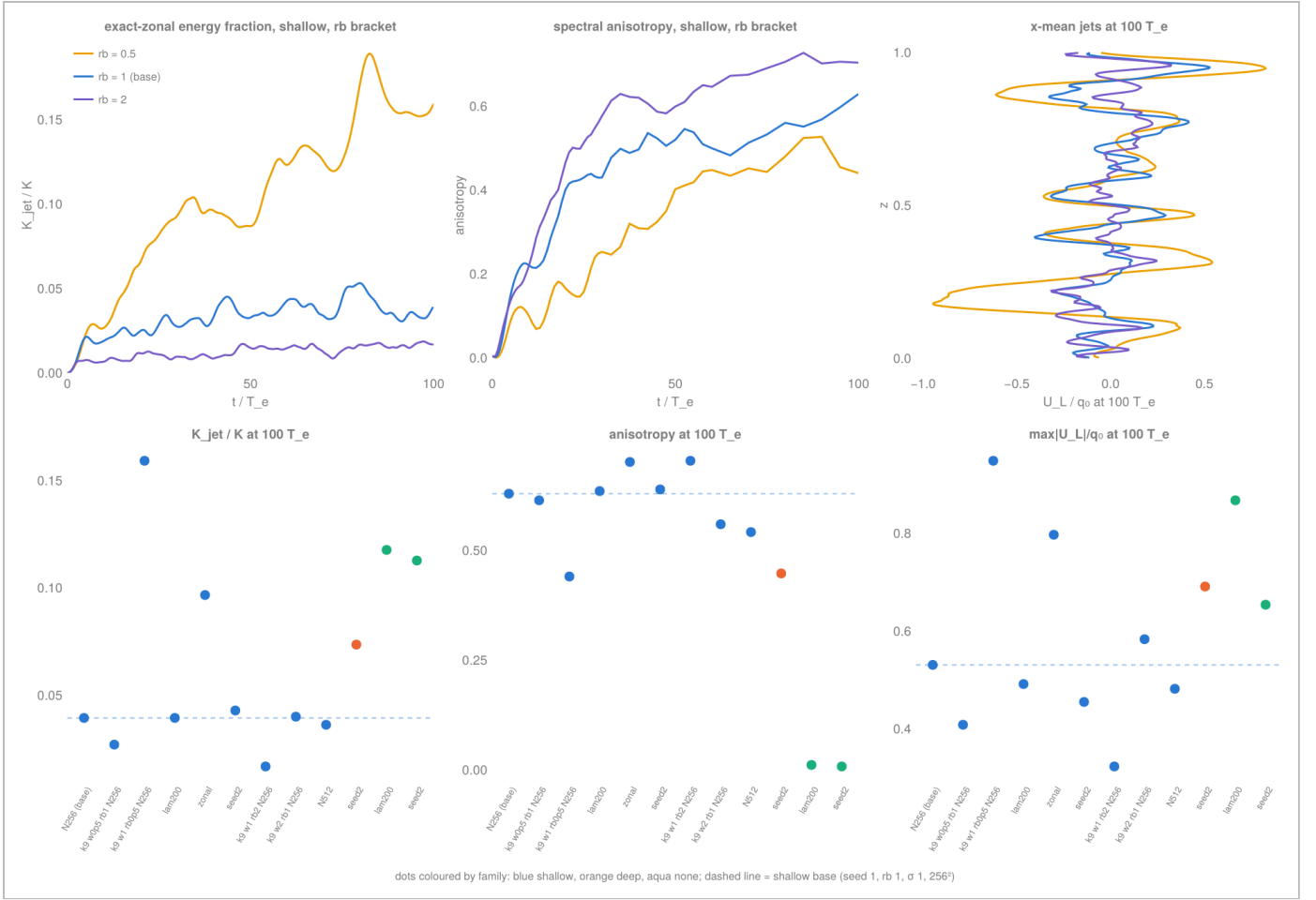
Sensitivity at 100 T_e . Top: the rb bracket for shallow waves — exact-zonal fraction 0.159 (rb = 0.5), \approx 0.04 (rb = 1), 0.017 (rb = 2) while the anisotropy index runs the other way (0.44, 0.62, 0.70): a stronger \beta arrests the cascade nearer the ring and keeps the energy in zonally elongated waves rather than jets. Bottom: every variant at 100 T_e , coloured by family — ring width 0.5–2 modes, 512 2 , seed 2 and the \lambda = 200 rescaling ( u'_{\text{rms},0} = 0.031 , identical physics in the nonlinear WENO regime: 0.039 vs \approx 0.04 , with 1% energy loss instead of +0.03%) all sit within the scatter; keeping the k_x = 0 modes adds their 6% almost additively (0.097); deep seed 2 gives 0.074 against \approx 0.2 for seed 1. Figure final_variants.png .
