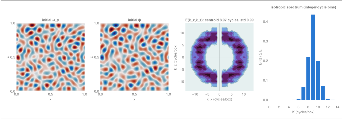
Shared initial condition ( 256^2 ): \omega_y , \psi , E(k_x, k_z) and the isotropic spectrum. Centroid 8.97 cycles, standard deviation 0.99, divergence 7e-18 , w = \omega_y = 0 on the walls, anisotropy index 0.004 (0.057 if the k_x = 0 modes were kept). u'_{rms,0} = 1.56e-4 , K = 1.22e-8 , enstrophy 7.84e-5 . Figure final_ic.png.
