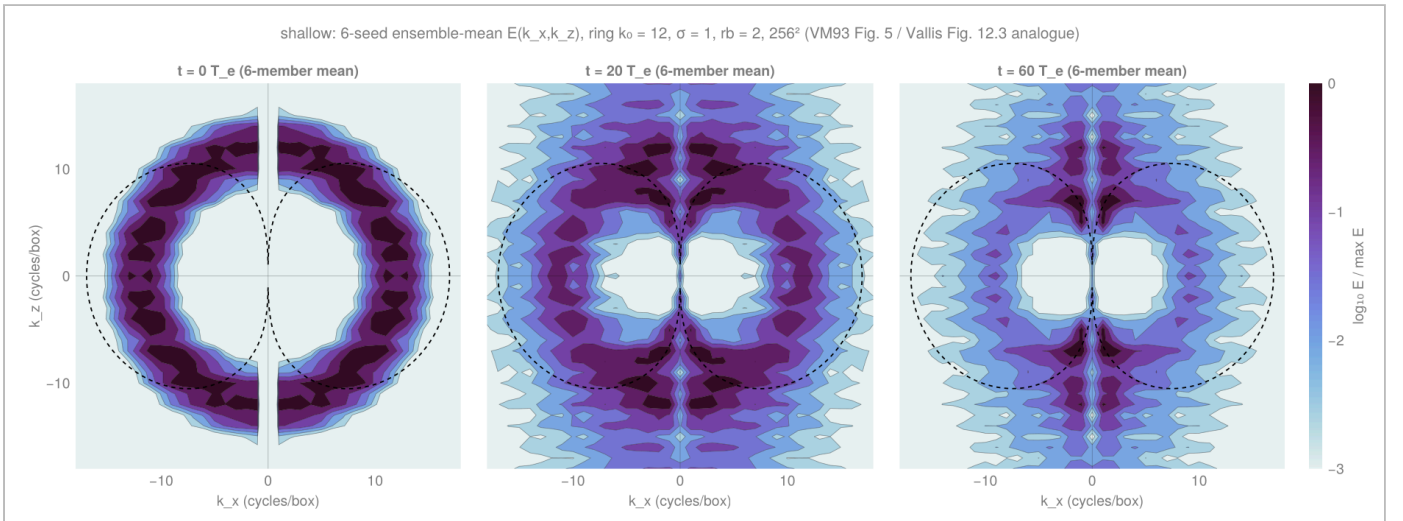
VM93 Fig. 5 / Vallis Fig. 12.3 analogue. Six-seed ensemble mean E(k_x, k_z) for shallow waves with VM93-inspired parameters ( k_0 = 12 , \sigma = 1 , rb = 2 , 256 2 (VM93 Fig. 5 / Vallis Fig. 12.3 analogue)) at 0, 20 and 60 T_e (VM93's panels sit at \approx 0 , 17 and 50 turnovers). The energy leaves the ring, avoids the interior of the dashed Rhines-estimate dumbbell (hole around the k_x axis) and concentrates at the poles, forming a narrow hourglass along k_z by 60 T_e ; the dashed curve is the velocity-based Rhines estimate, not the \epsilon -based Eq. 12.14 contour. Exact-zonal fraction 0.012 \pm 0.003 — small, as VM93 noted for the wave regime. Figure final_ensemble_spectra_shallow.png .
