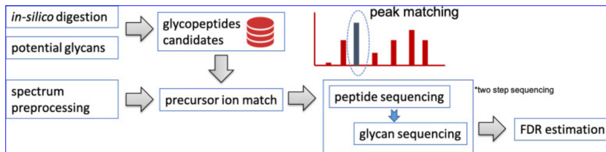
Figure 1. Workflow of the GlycoHybridSeq algorithm.
