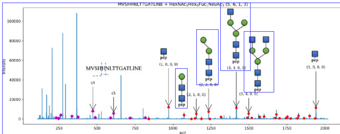
Figure 2. An example of annotated glycopeptide spectrum, where peaks annotated as b/c/y/z ions are colored as purple, and those annotated as Y ions as red.
