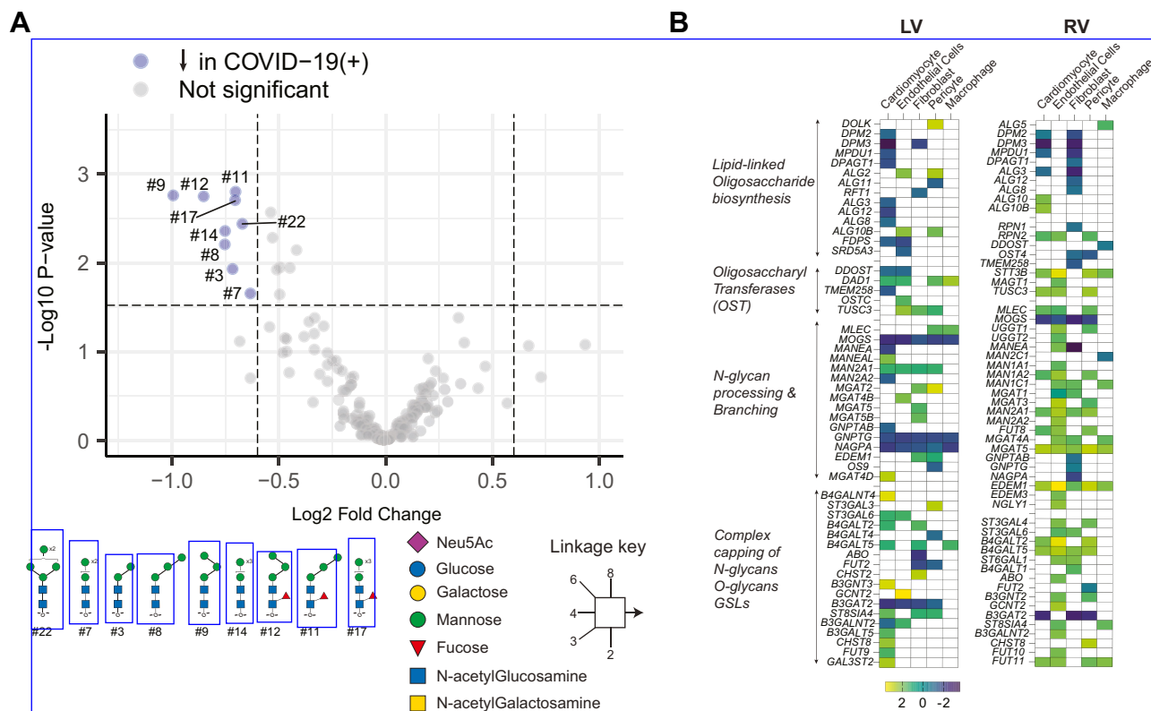
FIG. 6. Differences in FFPE tissue N -glycans that are independent of confounding variables. A, median normalized data were subjected to multivariate analysis to determine glycosylation changes independent of confounding factors such as age, sex, and comorbidities. Volcano plot represents differential abundance of glycans between COVID-19(-) and COVID-19(+) groups. Paucimannoses were reduced exclusively due to COVID-19. B, heat map representing \log_2 \text{FC} changes in expression of various enzymes in N -glycan biosynthesis obtained from snRNA-seq analysis (Fig. 1). LV-left ventricle, RV-right ventricle.
