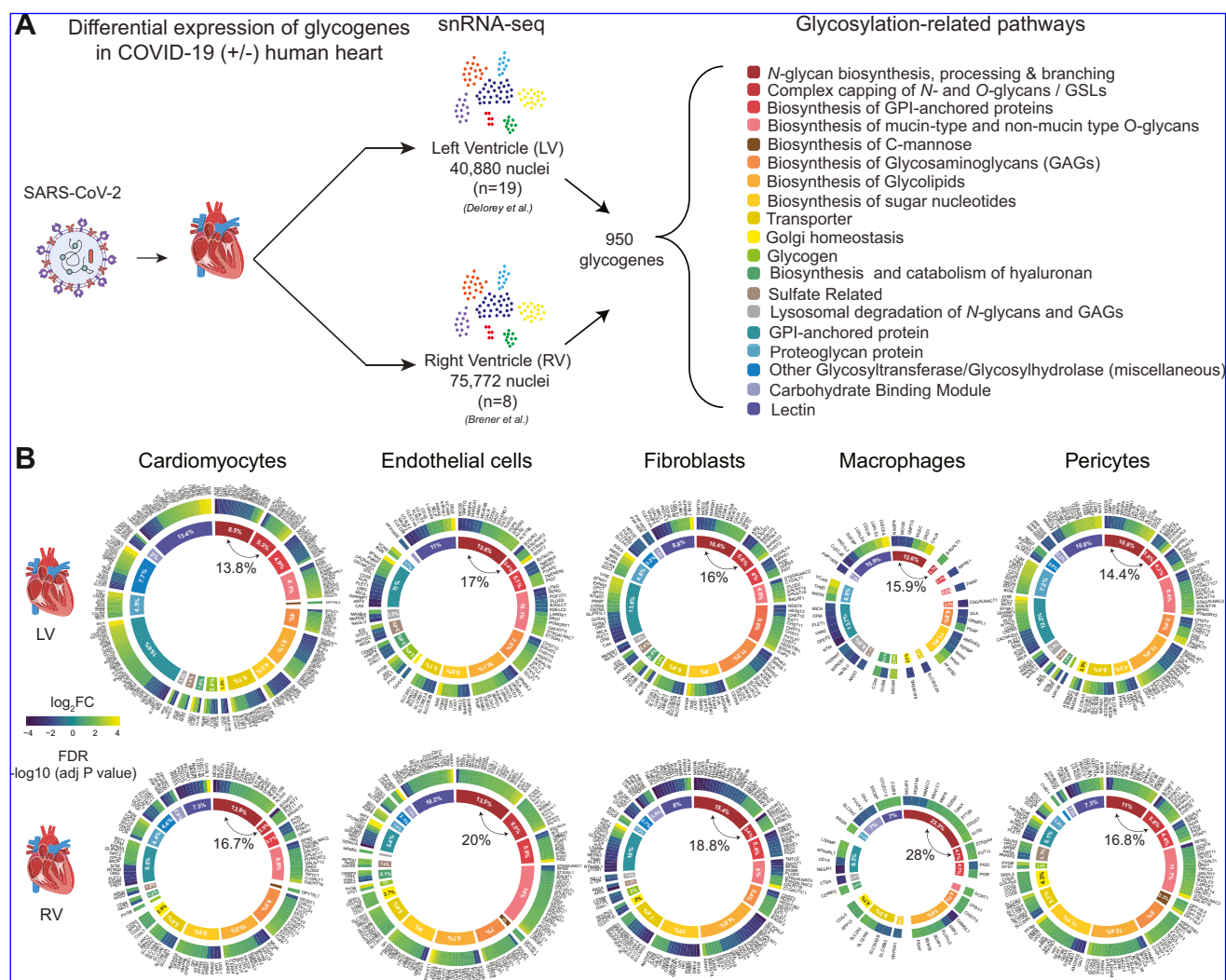
FIG. 1. Summary of snRNA-seq analysis of glycogenes in heart cells from COVID-19(+/) patients. A, schematic summary of the bioinformatic analysis of 950 glycosylation-related genes from 19 pathways interrogated from previously published snRNA-seq data (19, 20). B, relative distribution of glycogenes within individual cells of the left and right ventricular regions of the heart is presented as a radial heat map. The outer circle represents the gene expression profile of glycogenes having log2FC > \pm 1 and FDR < 0.05 . The inner circle represents the percentage contribution of each glycosylation-related pathway normalized to the total abundance. Glycogenes of N-glycan biosynthesis having 15 to 20% variation are indicated within the inner circle. The color gradients for the inner and outer circles in B correspond to the legend for glycosylation-related pathways in A and gene expression fold changes, respectively. Parts of this figure were generated with Biorender.com
