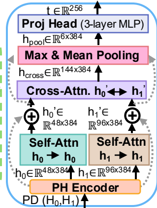
(b) Structure of H-Topo. Encoder
