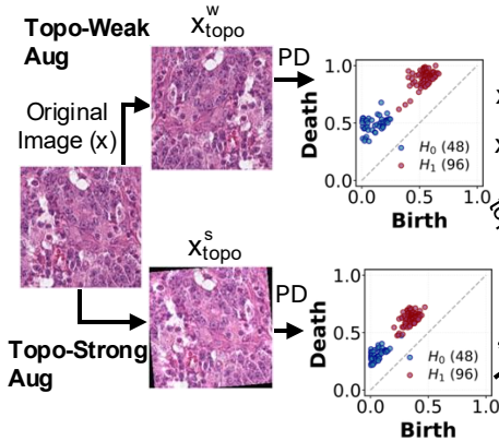
(a) Topological Contrastive Learning
