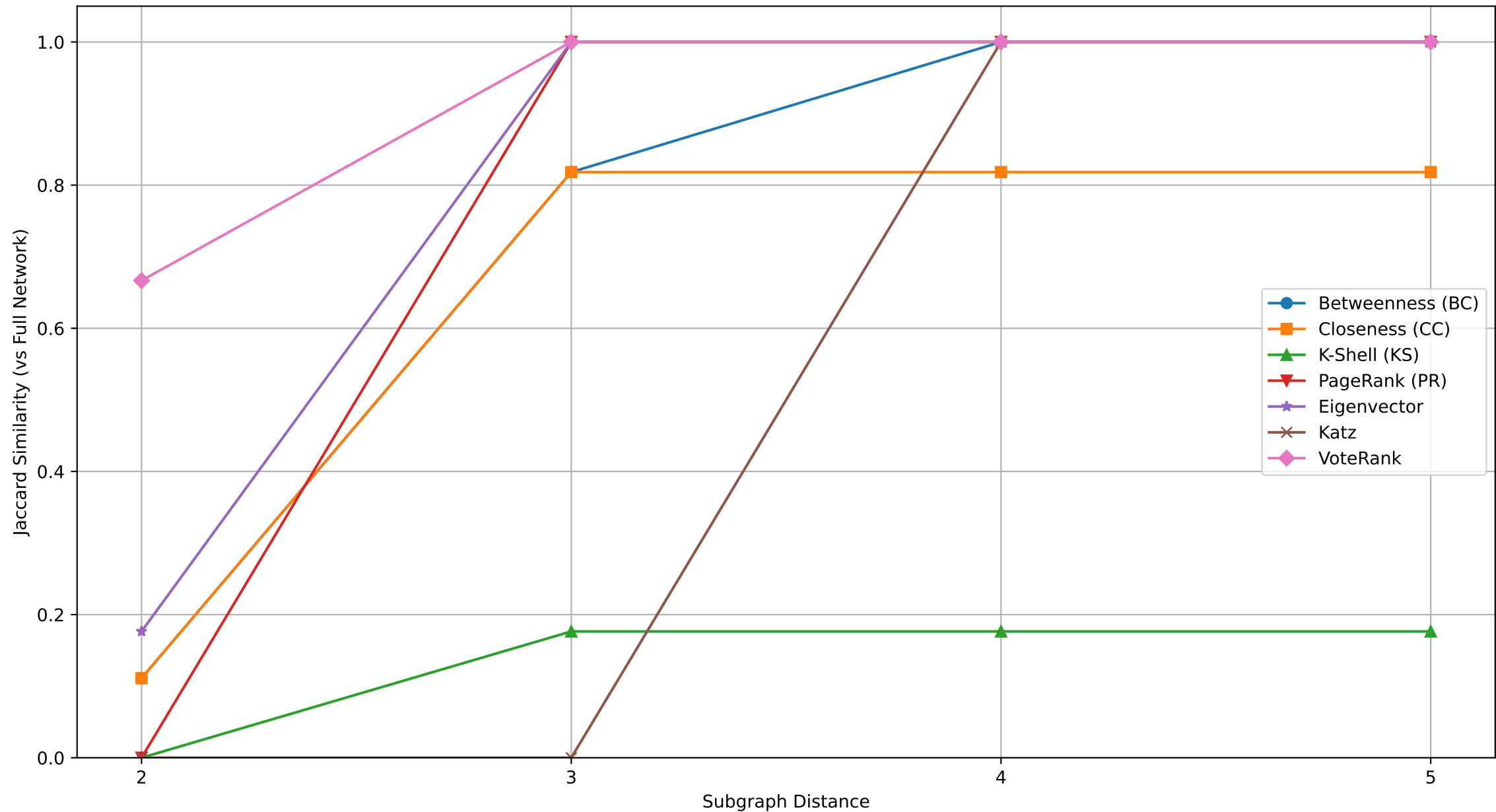
Physician (Top-10)
