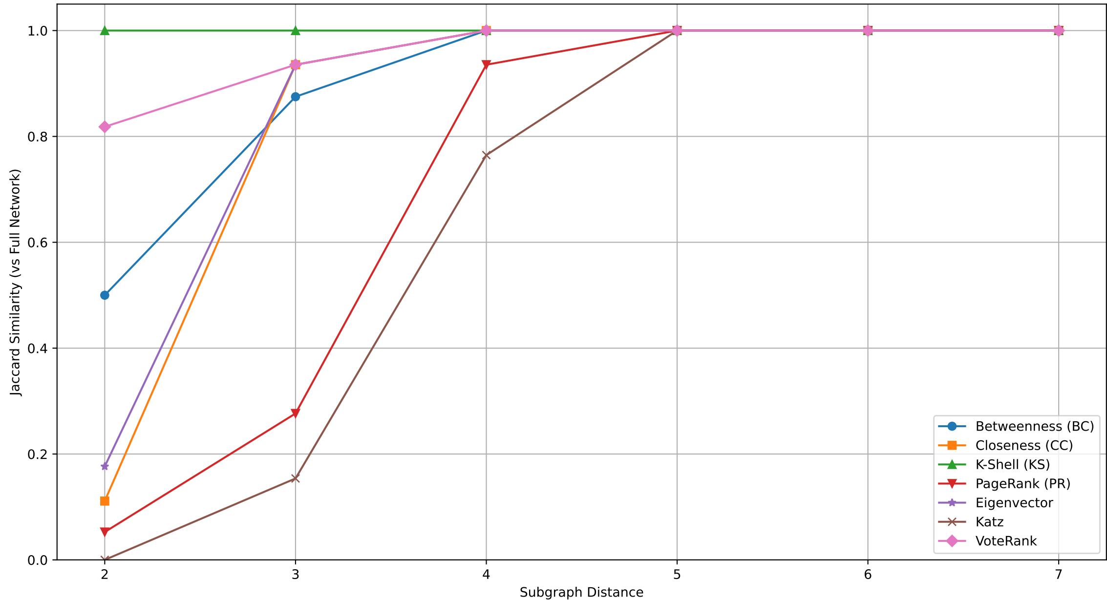
Celegans (Top-30)
