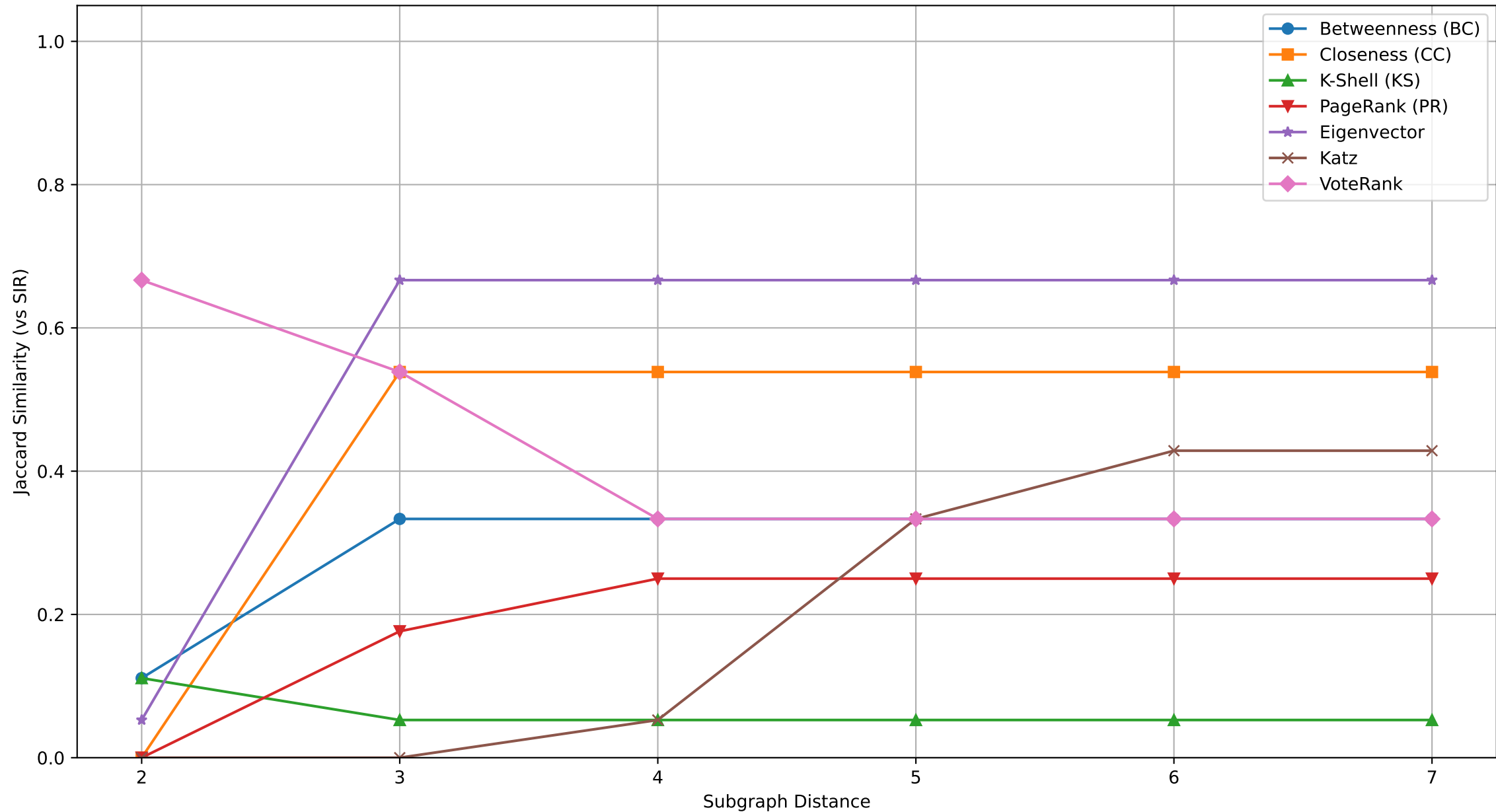
Unicode (Top-10)
