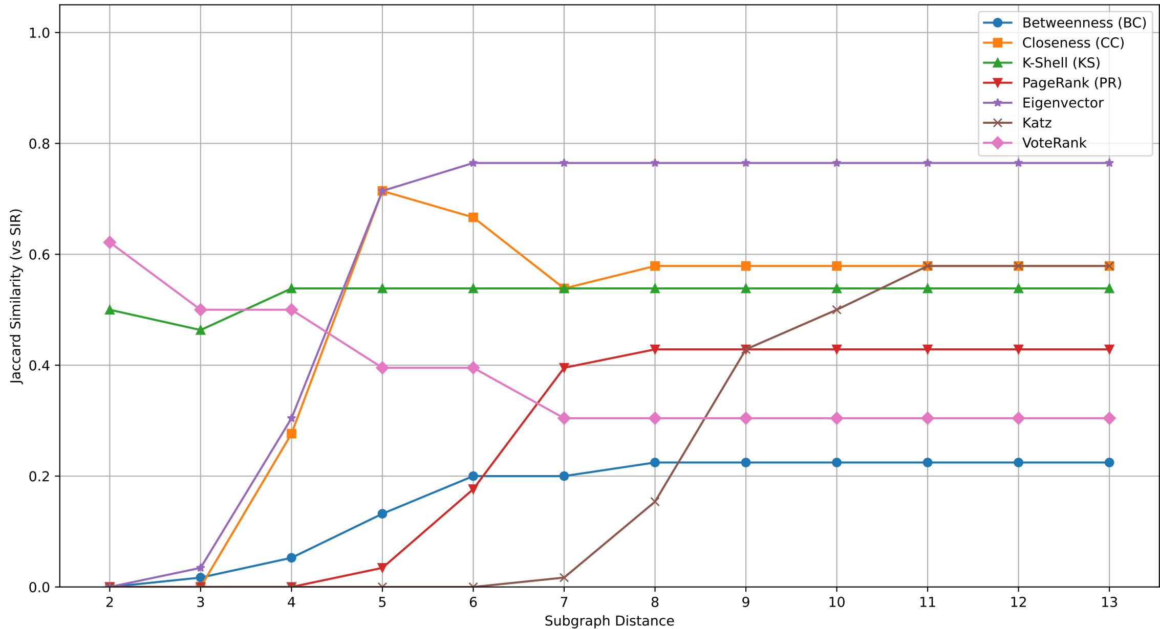
FilmTrust (Top-30)
