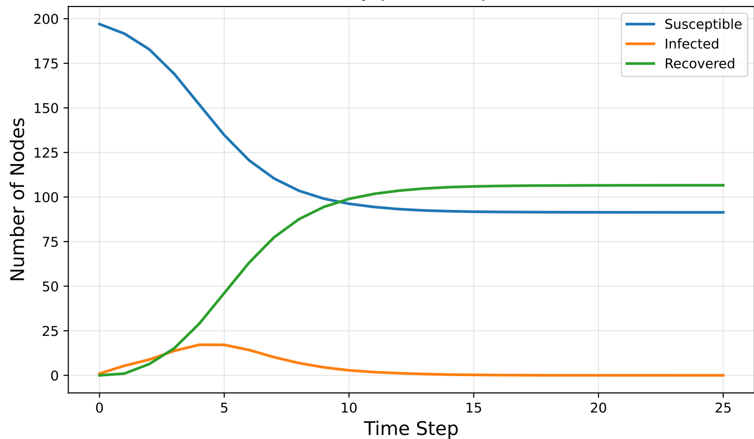
Betweenness Centrality ( \beta = 0.0531 , \mu = 1.0 , Seed = 67)
