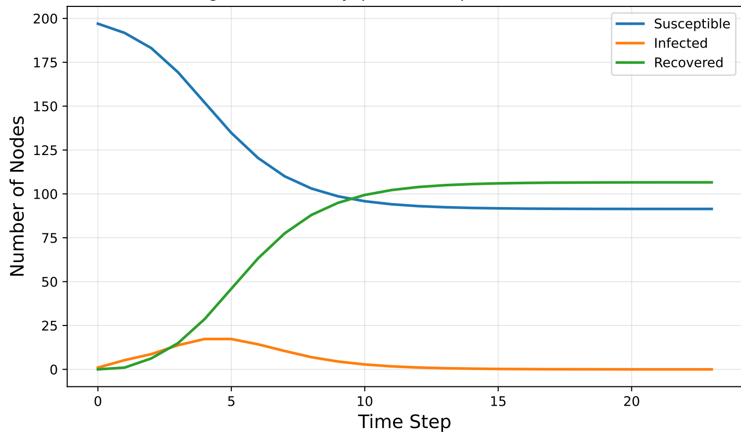
PageRank Centrality ( \beta = 0.0531 , \mu = 1.0 , Seed = 67)
