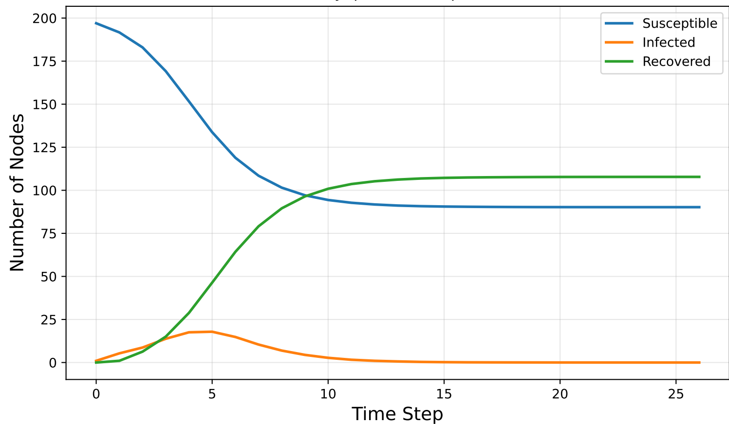
VoteRank Centrality ( \beta = 0.0531 , \mu = 1.0 , Seed = 67)
