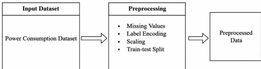
Figure 3.3: Pre-processing Overview
