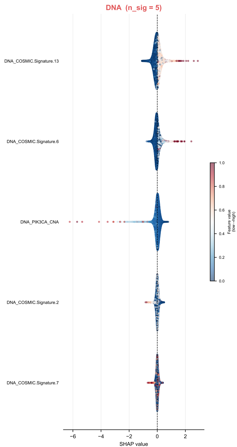
SHAP attribution — consensus signatures | Global Model Each point = one test patient · Colour: blue = low feature value, red = high · Restricted to features in the final consensus signature
