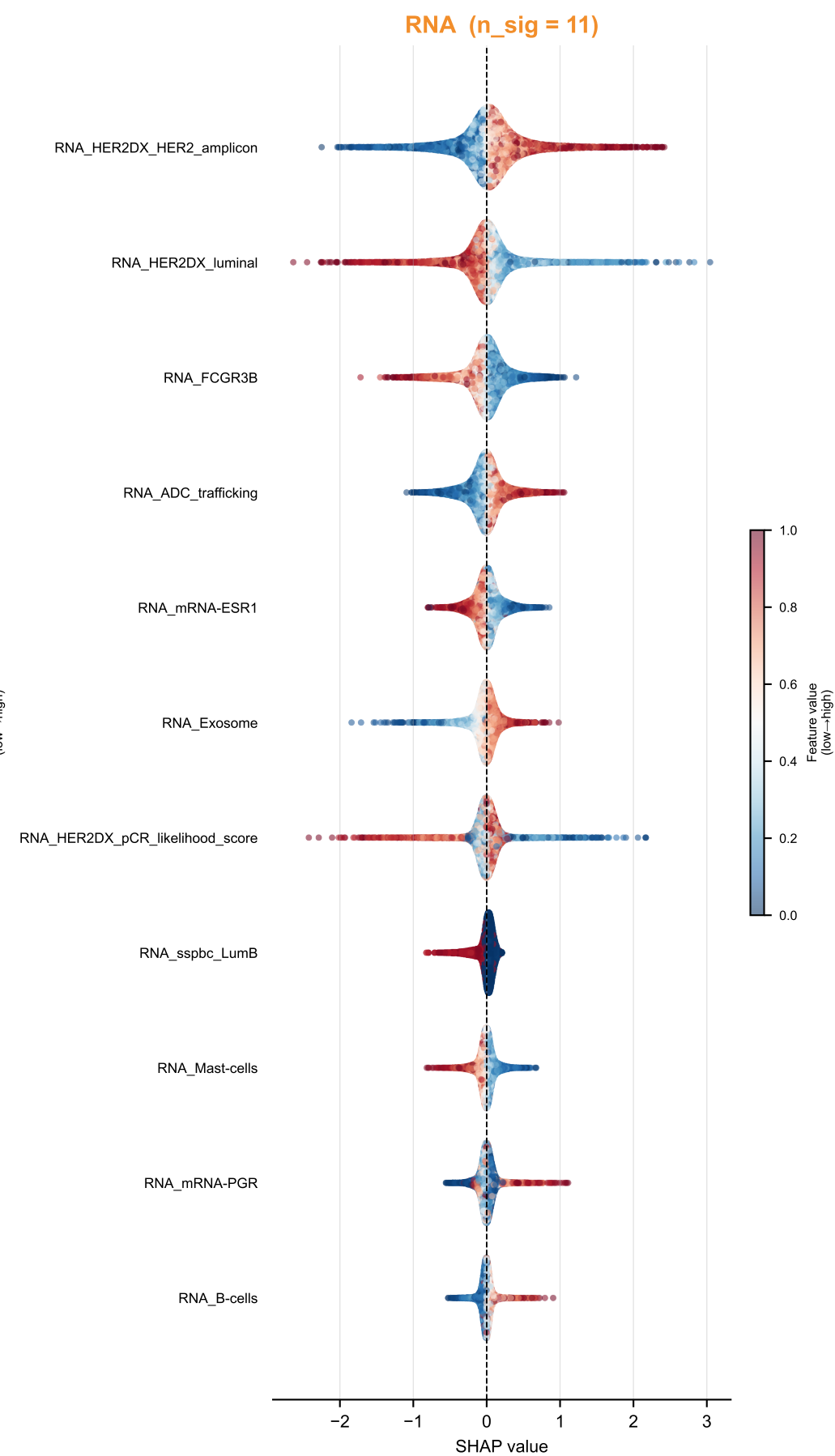
SHAP attribution — consensus signatures | Global Model Each point = one test patient · Colour: blue = low feature value, red = high · Restricted to features in the final consensus signature
