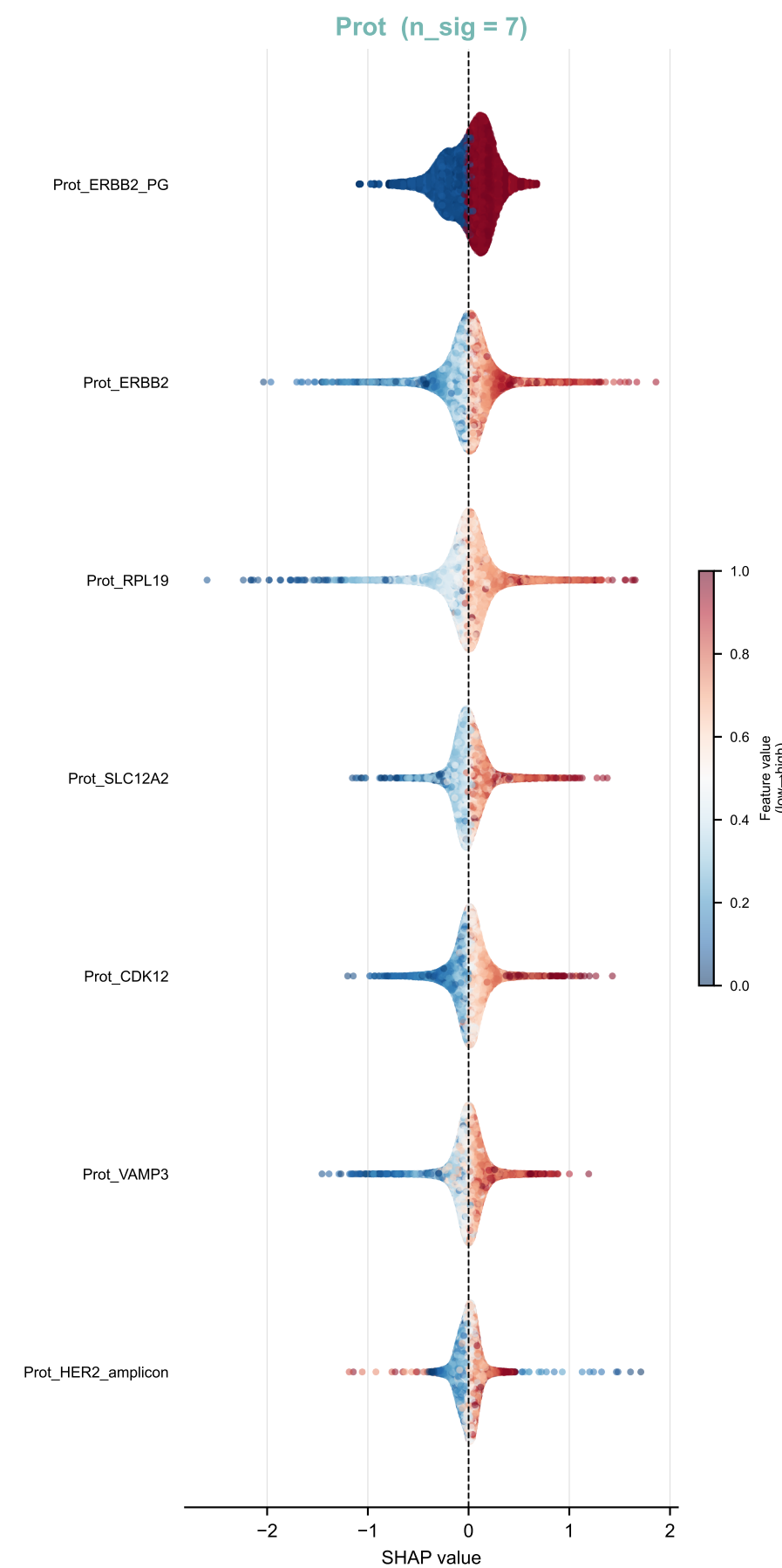
SHAP attribution — consensus signatures | Global Model Each point = one test patient · Colour: blue = low feature value, red = high · Restricted to features in the final consensus signature
