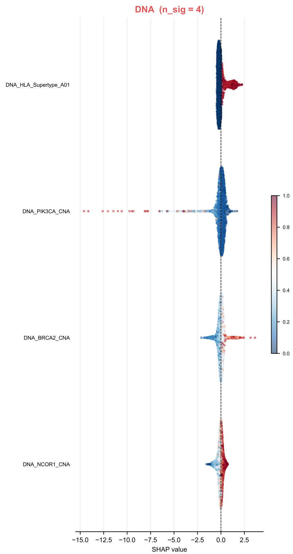
SHAP attribution — consensus signatures | T-DM1 Arm Each point = one test patient · Colour: blue = low feature value, red = high · Restricted to features in the final consensus signature
