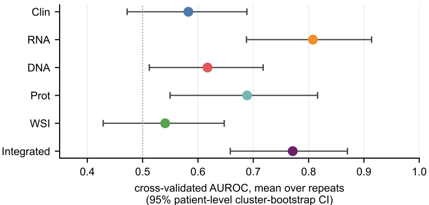
T-DM1 — performance
