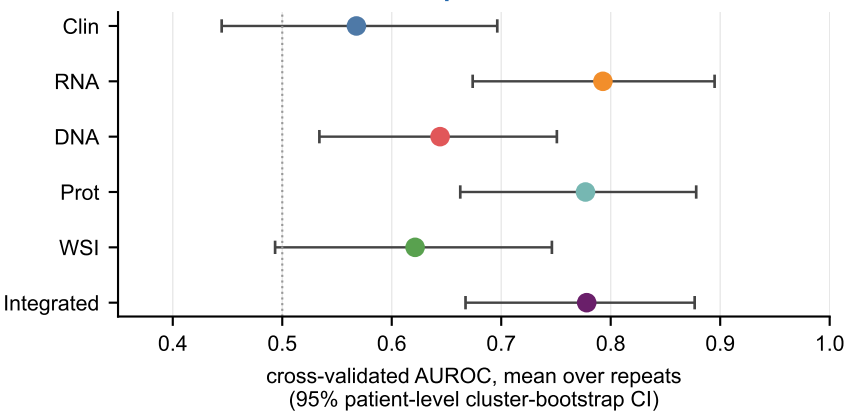
T-DM1 — performance
