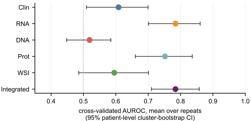
DHP — performance
