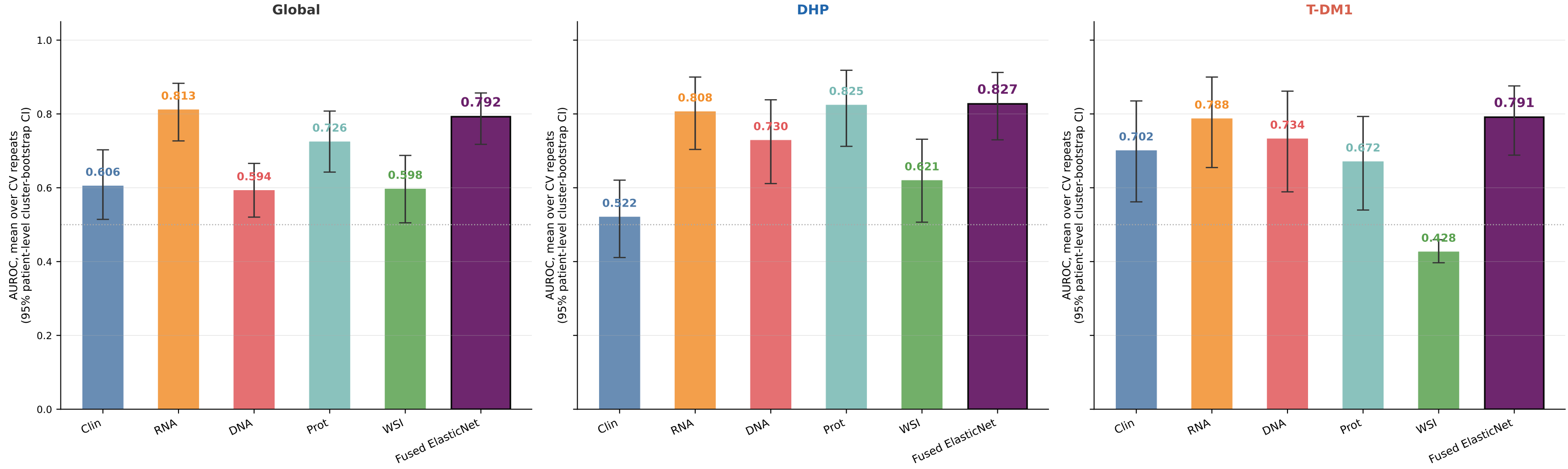
Consensus-signature performance — iterated outer CV AUROC, mean over CV repeats (95% patient-level cluster-bootstrap CI) · signature frozen, classifier + fusion refit within each fold
