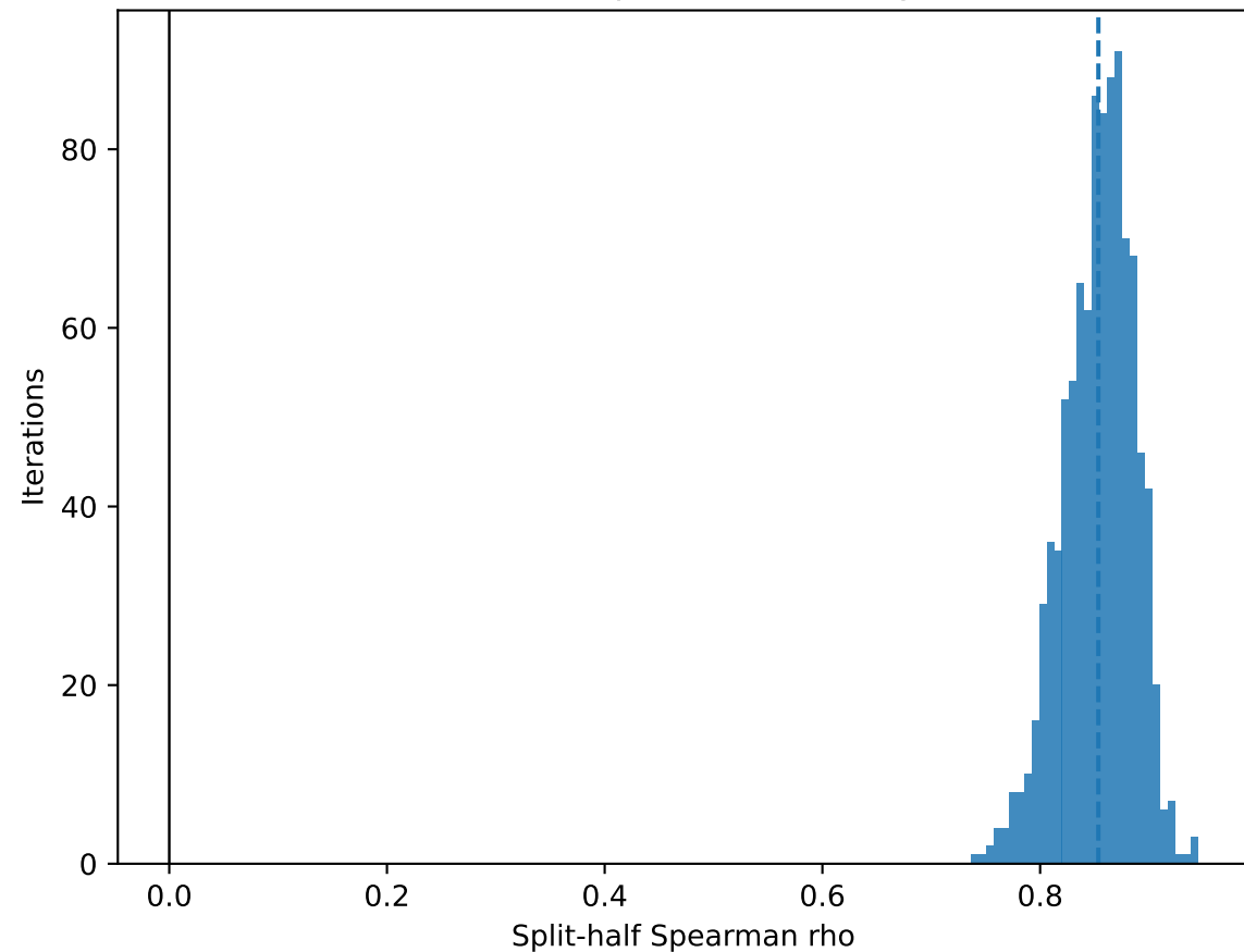
ResCLIP split-half reliability
