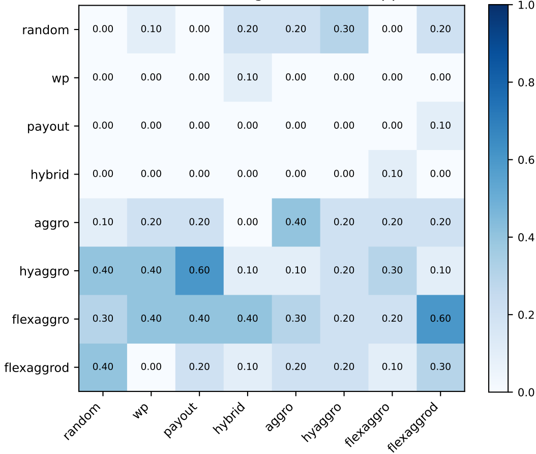
Win rate (rows = target, cols = 3×opponent)
