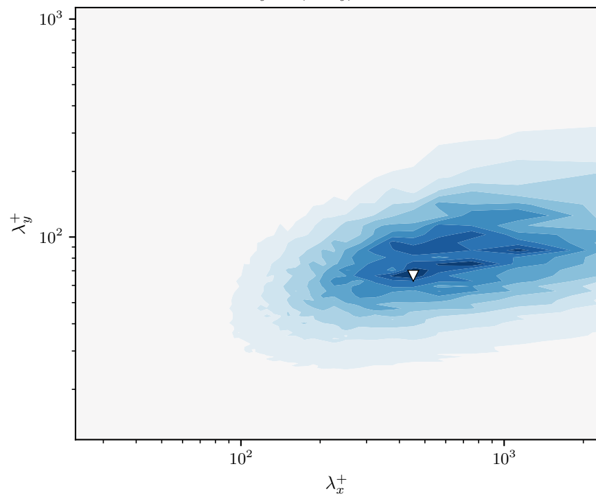
k_x k_y E_{uw}(k_x, k_y) at z^+ \approx 15
