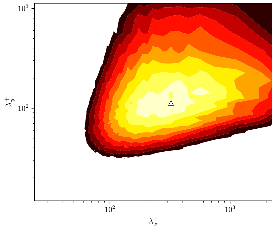
k_x k_y E_{vv}(k_x, k_y) at z^+ \approx 15
