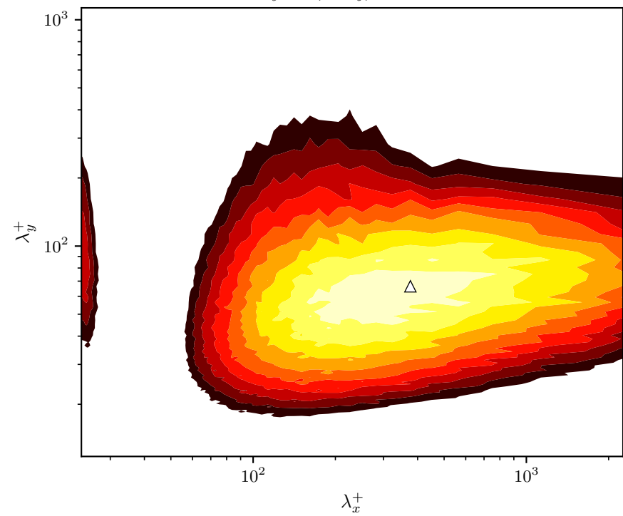
k_x k_y E_{ww}(k_x, k_y) at z^+ \approx 15
