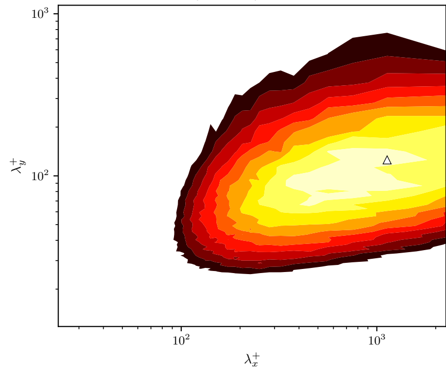
k_x k_y E_{uu}(k_x, k_y) at z^+ \approx 15
