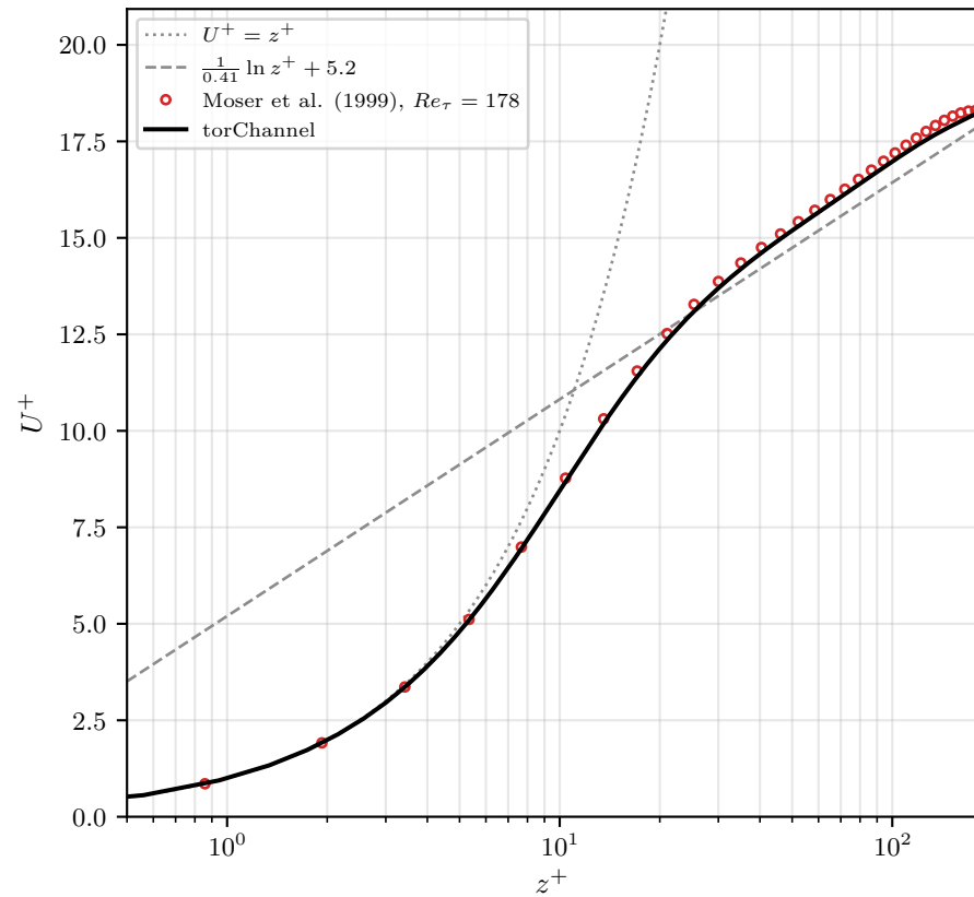
Mean Velocity Profile
