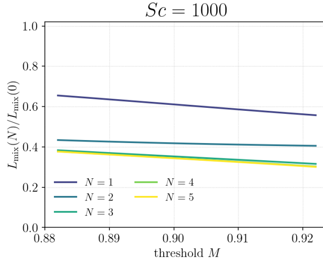
Figure 5: Threshold sensitivity at Sc = 1000 ( N = 1 – 5 , same quantity as Fig. 4). The reachable band is narrow ( M \gtrsim 0.88 ) because the L_x = 90 field mixes N = 0 only to M \approx 0.88 ; within it the ratio is again smooth and monotone with the same N -ordering, consistent with the lower- Sc panels.
