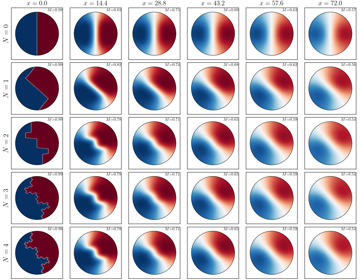
Figure 7: As Fig. 6 but at Sc = 100 ( N = 0 – 4 , stations x = 0 to 72 ). At the lower Pe the field mixes further within the domain (outlet M \approx 0.54 – 0.57 ); the same trend holds — the fractal striations diffuse out and higher N homogenises sooner.
