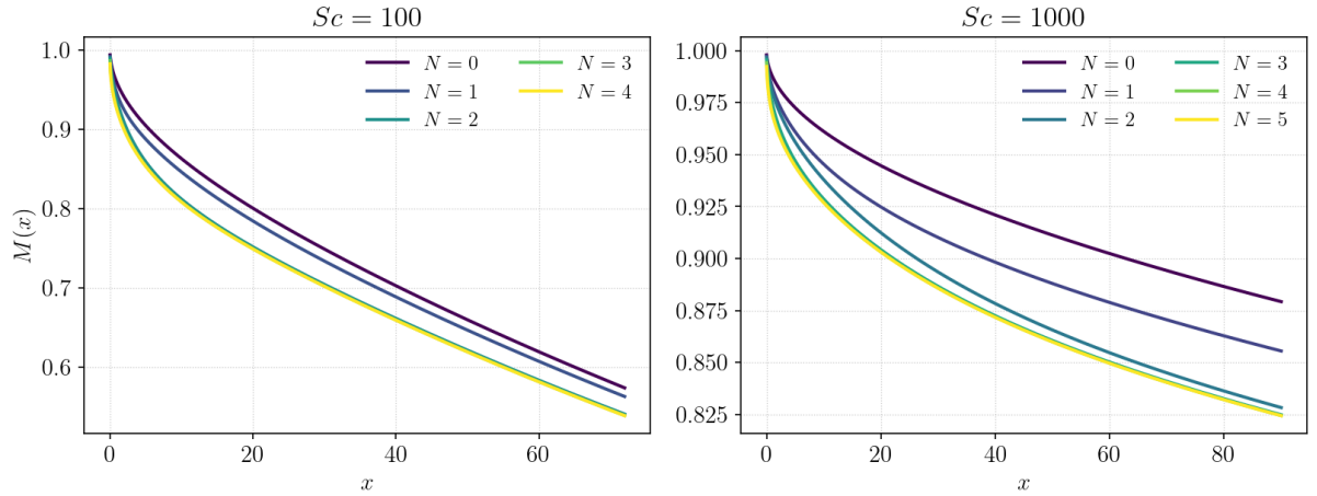
Figure 8: Segregation decay M(x) , generations N overlaid, for Sc = 100 ( L_x = 72 , left) and Sc = 1000 ( L_x = 90 , right). Higher N decays faster and further in both. Both cross M = 0.9 within their domains, so the mixing length is read at the same threshold for every Sc (Table 1).
