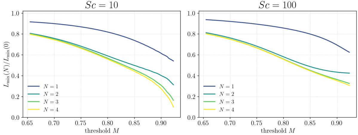
Figure 4: Threshold sensitivity of the ratio L_{\text{mix}}(N)/L_{\text{mix}}(0) : each curve is a generation N (colour as in Fig. 8) swept over the mixedness threshold M . The ratio rises smoothly and monotonically toward 1 as M is lowered — it never flickers or reverses — and the N -ordering is preserved at every M . The fractal advantage is therefore largest near the inlet (high M ) and fades toward complete mixing, but the qualitative conclusions are threshold-independent; only the reported magnitude depends on the chosen M . Over the same range the Sc = 10 and Sc = 100 panels have nearly the same shape, confirming the behaviour is not Sc -specific (see also Sc = 1000 , Fig. 5).
