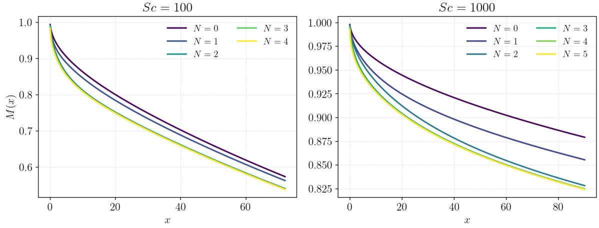
Figure 6: Segregation decay M(x) , generations N overlaid, for Sc = 100 ( L_x = 72 , left) and Sc = 1000 ( L_x = 90 , right). Higher N decays faster and further in both. Both cross M = 0.9 within their domains, so the mixing length is read at the same threshold for every Sc (Table 1).
