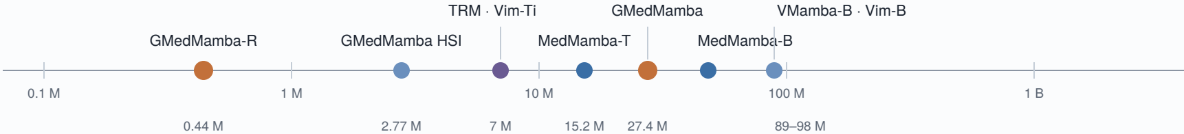
Parameter scale (log), same axis for every model above
