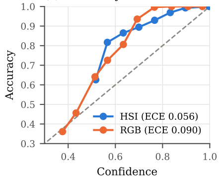
(c) Reliability, test, seed 42
