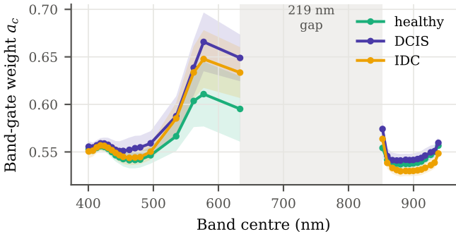
(a) Learned band gate ( \pm 1 s.d.)
