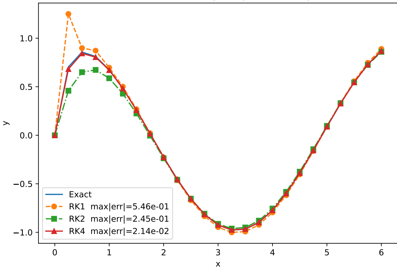
RK1 vs RK2 vs RK4 on y' + 5y = 5 \cos x , y(0)=0
