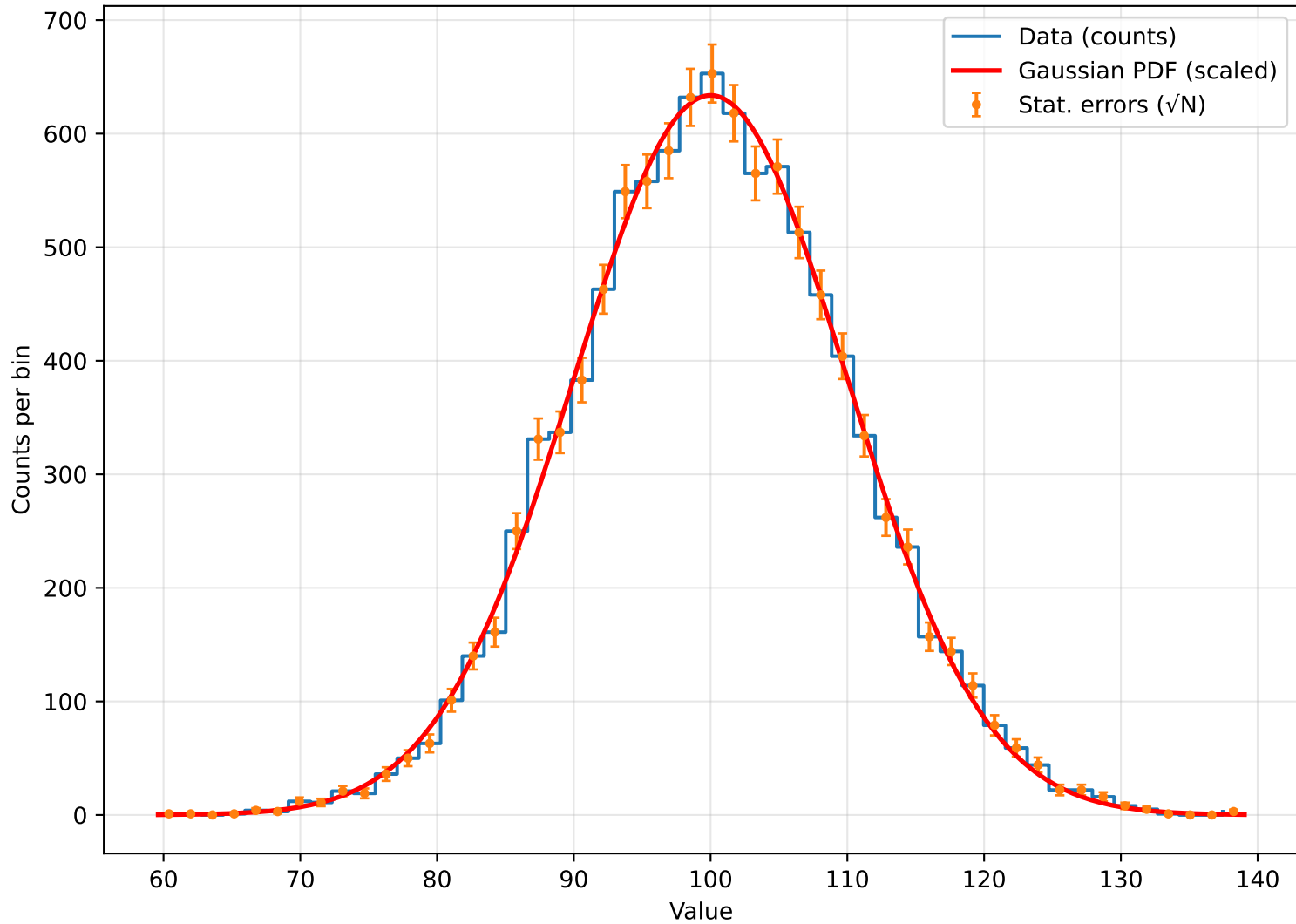
Canvas 2 (Matplotlib)
