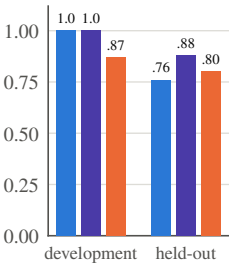
top-1 accuracy
