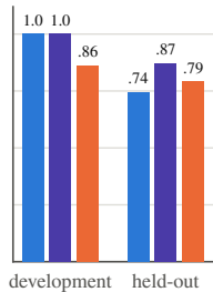
Cohen's \kappa
