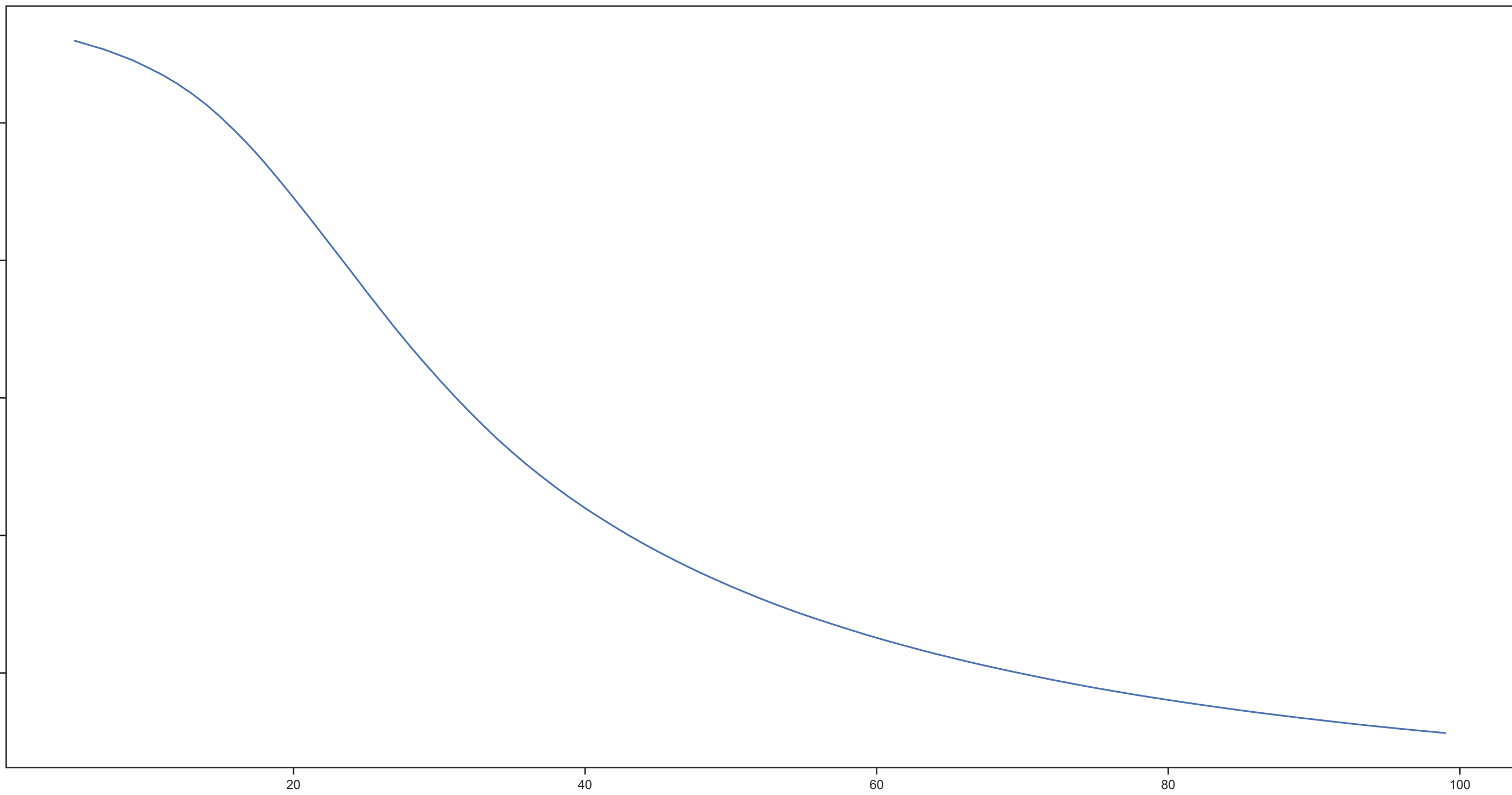
DAE loss
