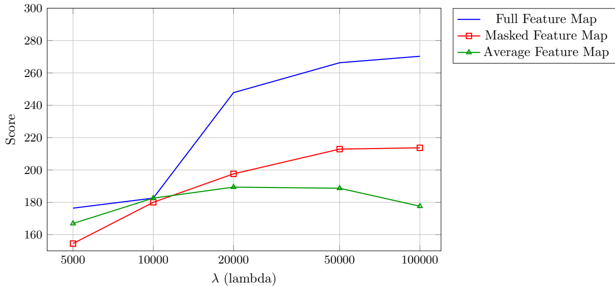
IS vs. \lambda
