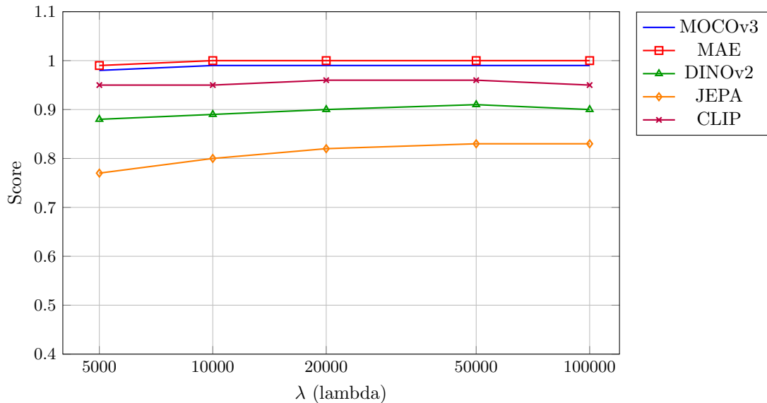
Average Feature Map Scores vs. \lambda
