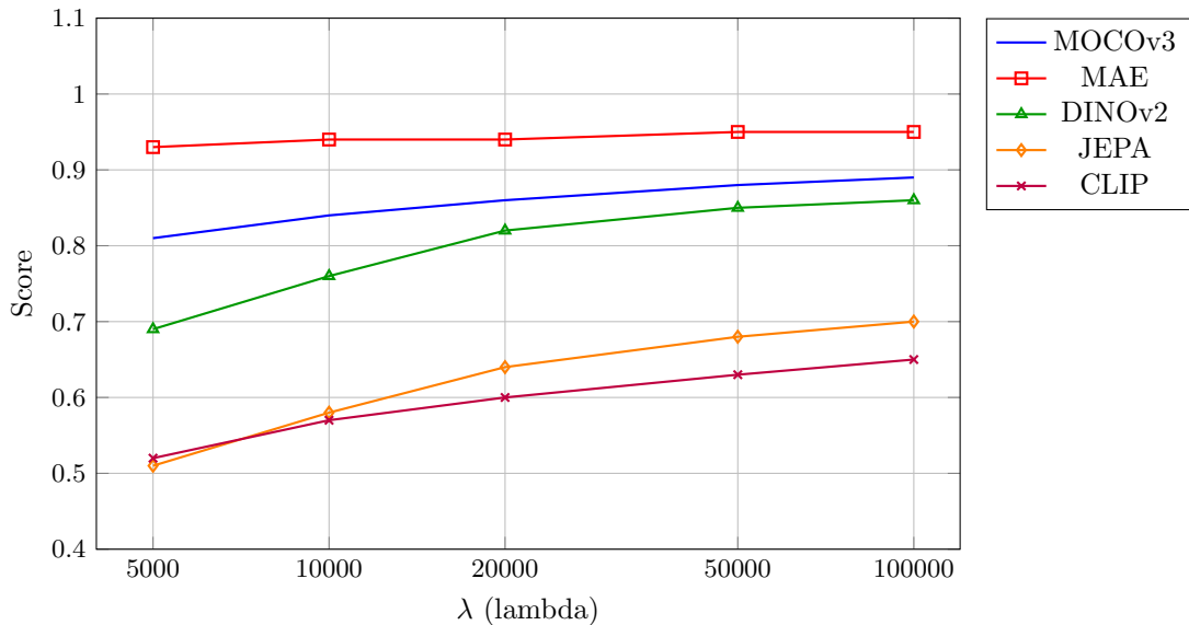
Masked Feature Map Scores vs. \lambda
