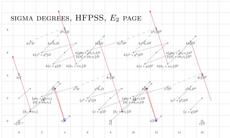
Fig. 13 The E_2 -page of the (* - \sigma_i) -graded Q_8 -HFPSS( \mathbf{E}_2 ). The lines of slope-3 are d_3 -differentials
