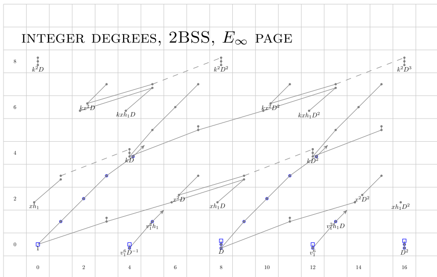
Fig. 3 The E_\infty -page of the integer-graded 2BSS. The dotted lines are hidden h_2 extensions
