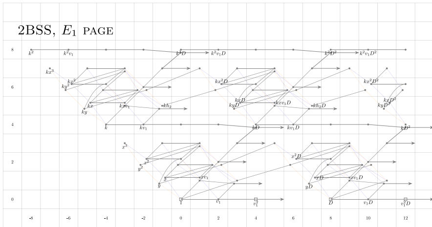
Fig. 2 The E_1 -page of the integer/ (* - \sigma_i) -graded 2BSS
