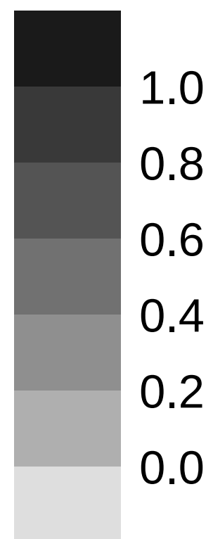
R_{\text{inv}} fold change
